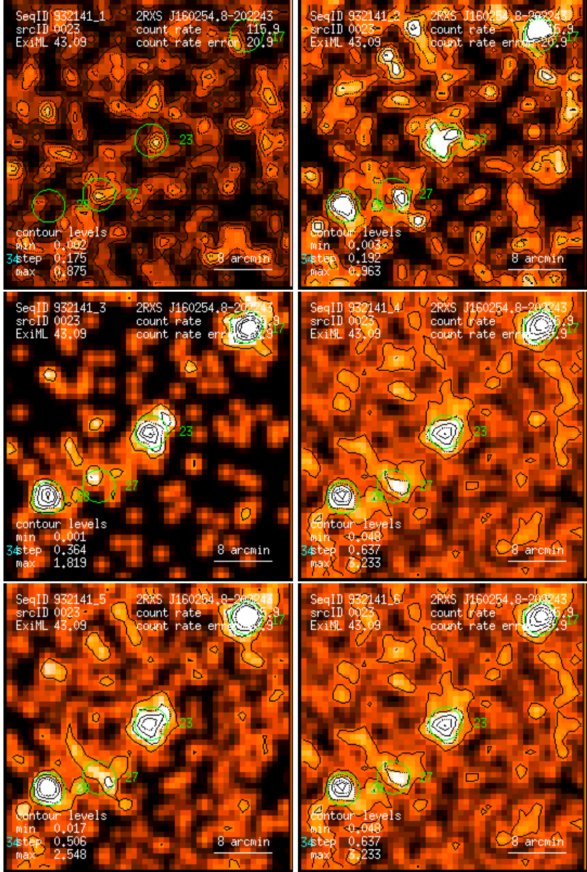
Figure 23: RASS 932141: detection 0023: band rate images, Gaussian filter: (1) PSPC channels 11 – 41, (2) 52 – 90, (3) 91 – 201, (4) 11 – 235, (5) 52 – 201, (6) 11 – 201. Broad band rates in counts/ks. Band rate contour levels in counts/ks/arcmin 2 .
