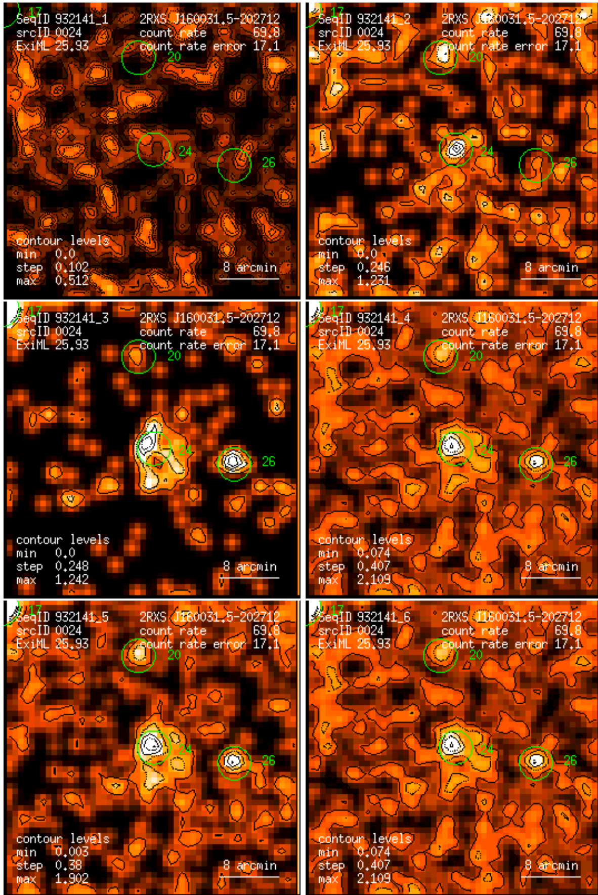
Figure 24: RASS 932141: detection 0024: band rate images, Gaussian filter: (1) PSPC channels 11 – 41, (2) 52 – 90, (3) 91 – 201, (4) 11 – 235, (5) 52 – 201, (6) 11 – 201. Broad band rates in counts/ks. Band rate contour levels in counts/ks/arcmin 2 .
