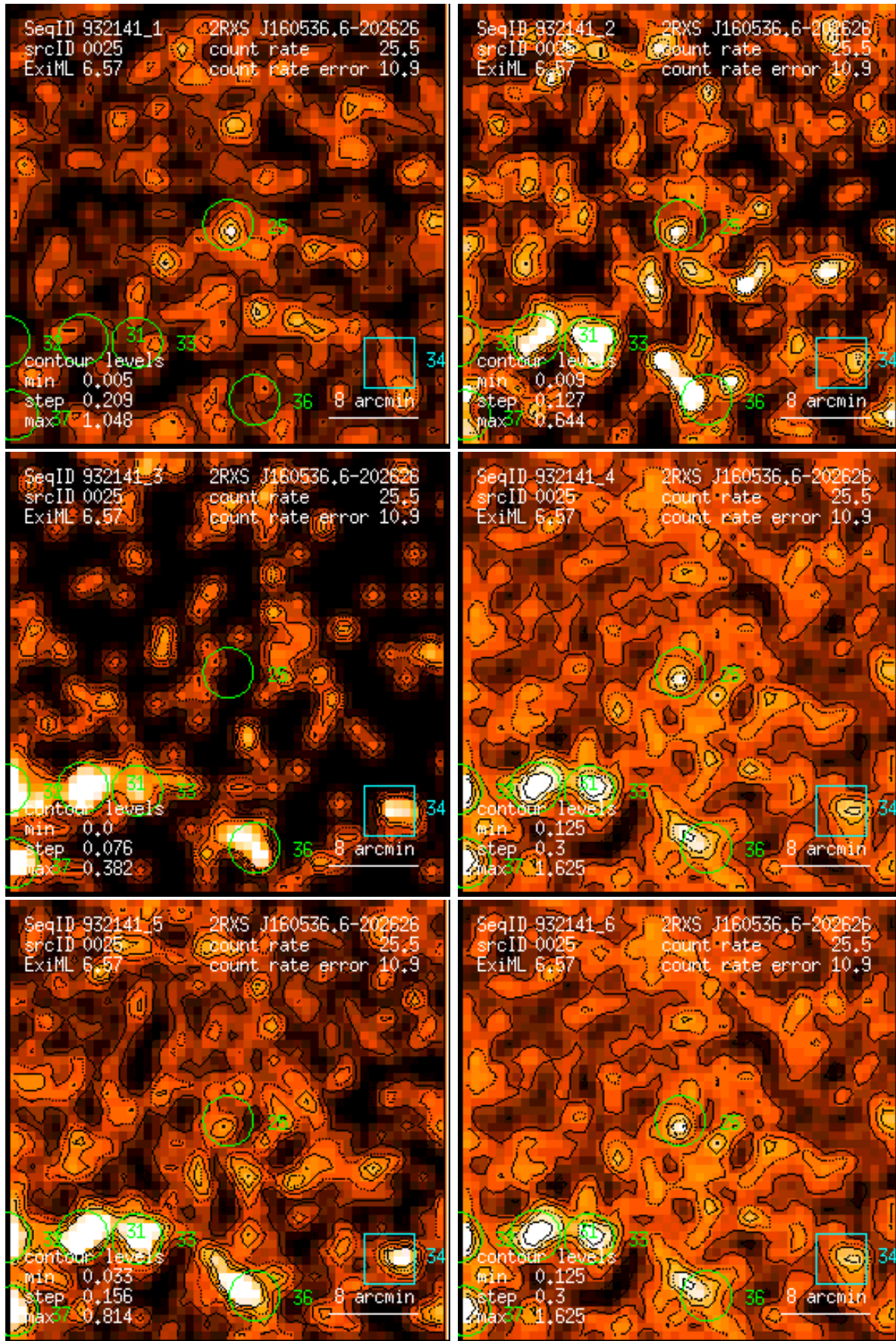
Figure 25: RASS 932141: detection 0025: band rate images, Gaussian filter: (1) PSPC channels 11 – 41, (2) 52 – 90, (3) 91 – 201, (4) 11 – 235, (5) 52 – 201, (6) 11 – 201. Broad band rates in counts/ks. Band rate contour levels in counts/ks/arcmin 2 .
