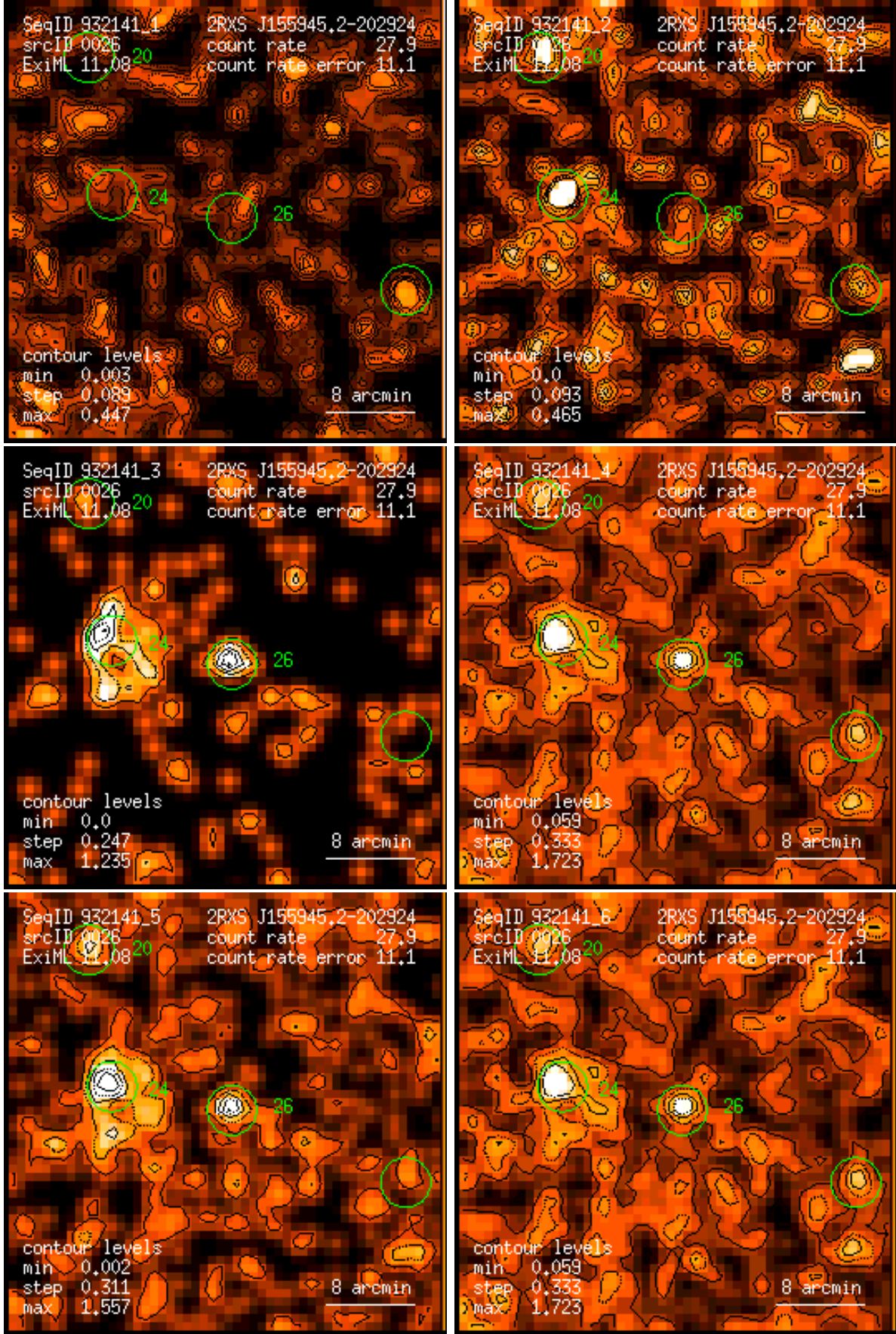
Figure 26: RASS 932141: detection 0026: band rate images, Gaussian filter: (1) PSPC channels 11 – 41, (2) 52 – 90, (3) 91 – 201, (4) 11 – 235, (5) 52 – 201, (6) 11 – 201. Broad band rates in counts/ks. Band rate contour levels in counts/ks/arcmin 2 .
