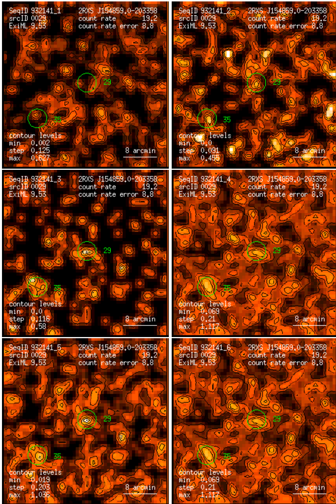
Figure 29: RASS 932141: detection 0029: band rate images, Gaussian filter: (1) PSPC channels 11 – 41, (2) 52 – 90, (3) 91 – 201, (4) 11 – 235, (5) 52 – 201, (6) 11 – 201. Broad band rates in counts/ks. Band rate contour levels in counts/ks/arcmin 2 .
