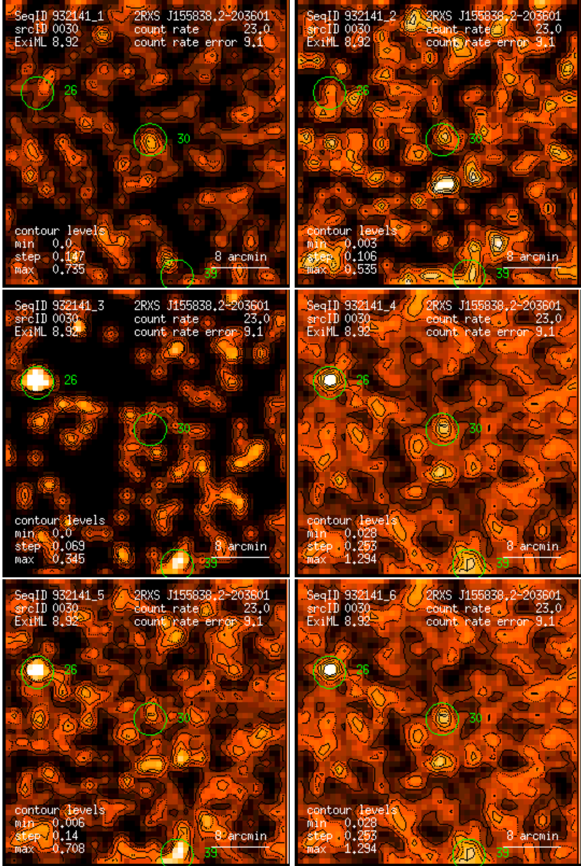
Figure 30: RASS 932141: detection 0030: band rate images, Gaussian filter: (1) PSPC channels 11 – 41, (2) 52 – 90, (3) 91 – 201, (4) 11 – 235, (5) 52 – 201, (6) 11 – 201. Broad band rates in counts/ks. Band rate contour levels in counts/ks/arcmin 2 .
