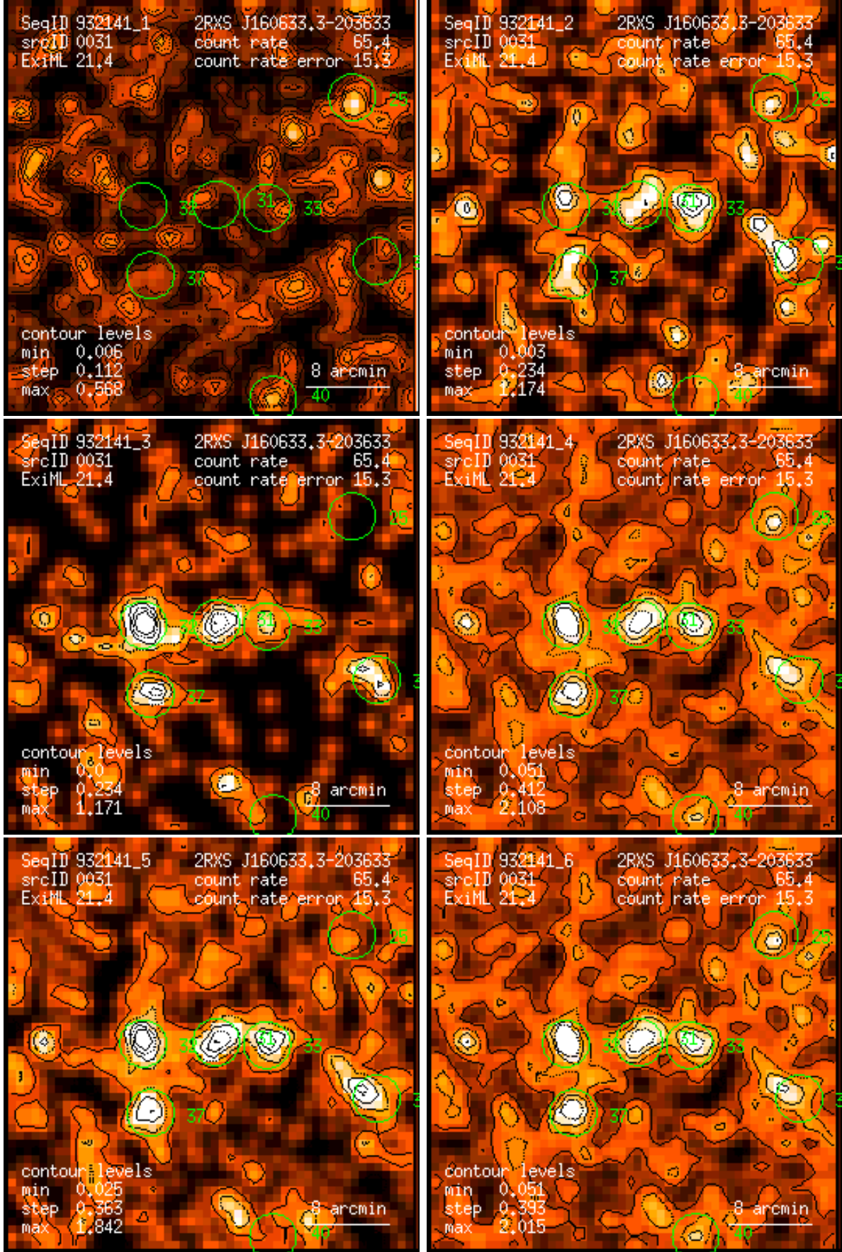
Figure 31: RASS 932141: detection 0031: band rate images, Gaussian filter: (1) PSPC channels 11 – 41, (2) 52 – 90, (3) 91 – 201, (4) 11 – 235, (5) 52 – 201, (6) 11 – 201. Broad band rates in counts/ks. Band rate contour levels in counts/ks/arcmin 2 .
