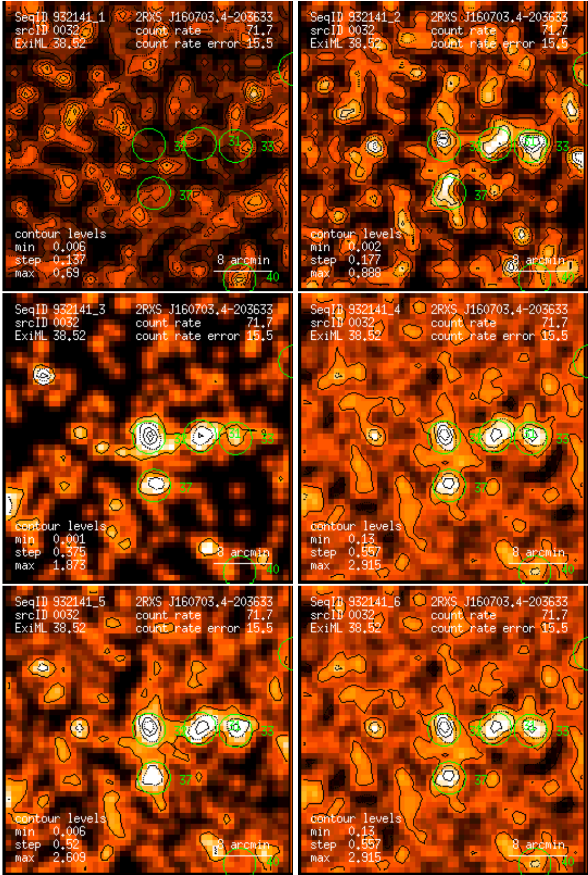
Figure 32: RASS 932141: detection 0032: band rate images, Gaussian filter: (1) PSPC channels 11 – 41, (2) 52 – 90, (3) 91 – 201, (4) 11 – 235, (5) 52 – 201, (6) 11 – 201. Broad band rates in counts/ks. Band rate contour levels in counts/ks/arcmin 2 .
