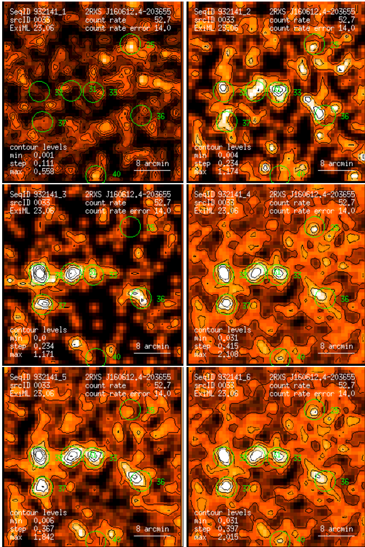
Figure 33: RASS 932141: detection 0033: band rate images, Gaussian filter: (1) PSPC channels 11 – 41, (2) 52 – 90, (3) 91 – 201, (4) 11 – 235, (5) 52 – 201, (6) 11 – 201. Broad band rates in counts/ks. Band rate contour levels in counts/ks/arcmin 2 .
