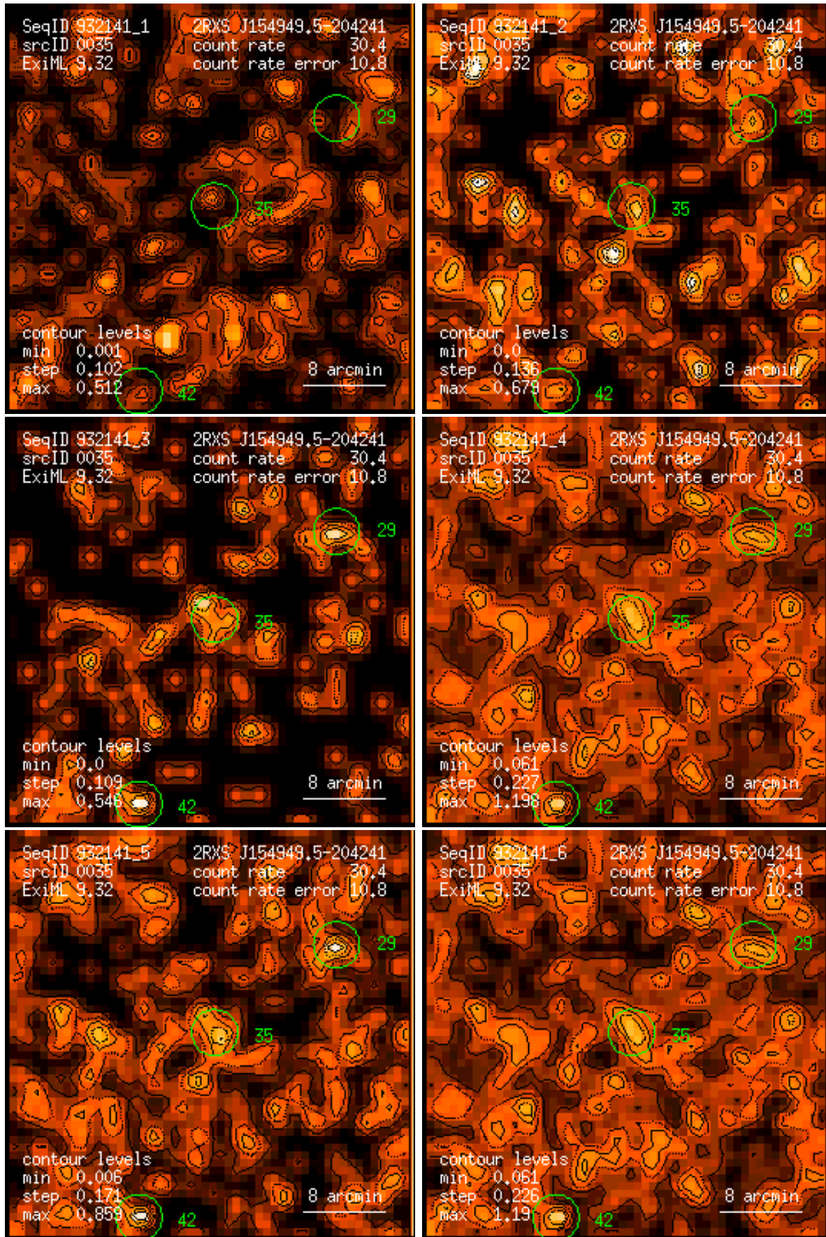
Figure 35: RASS 932141: detection 0035: band rate images, Gaussian filter: (1) PSPC channels 11 – 41, (2) 52 – 90, (3) 91 – 201, (4) 11 – 235, (5) 52 – 201, (6) 11 – 201. Broad band rates in counts/ks. Band rate contour levels in counts/ks/arcmin 2 .
