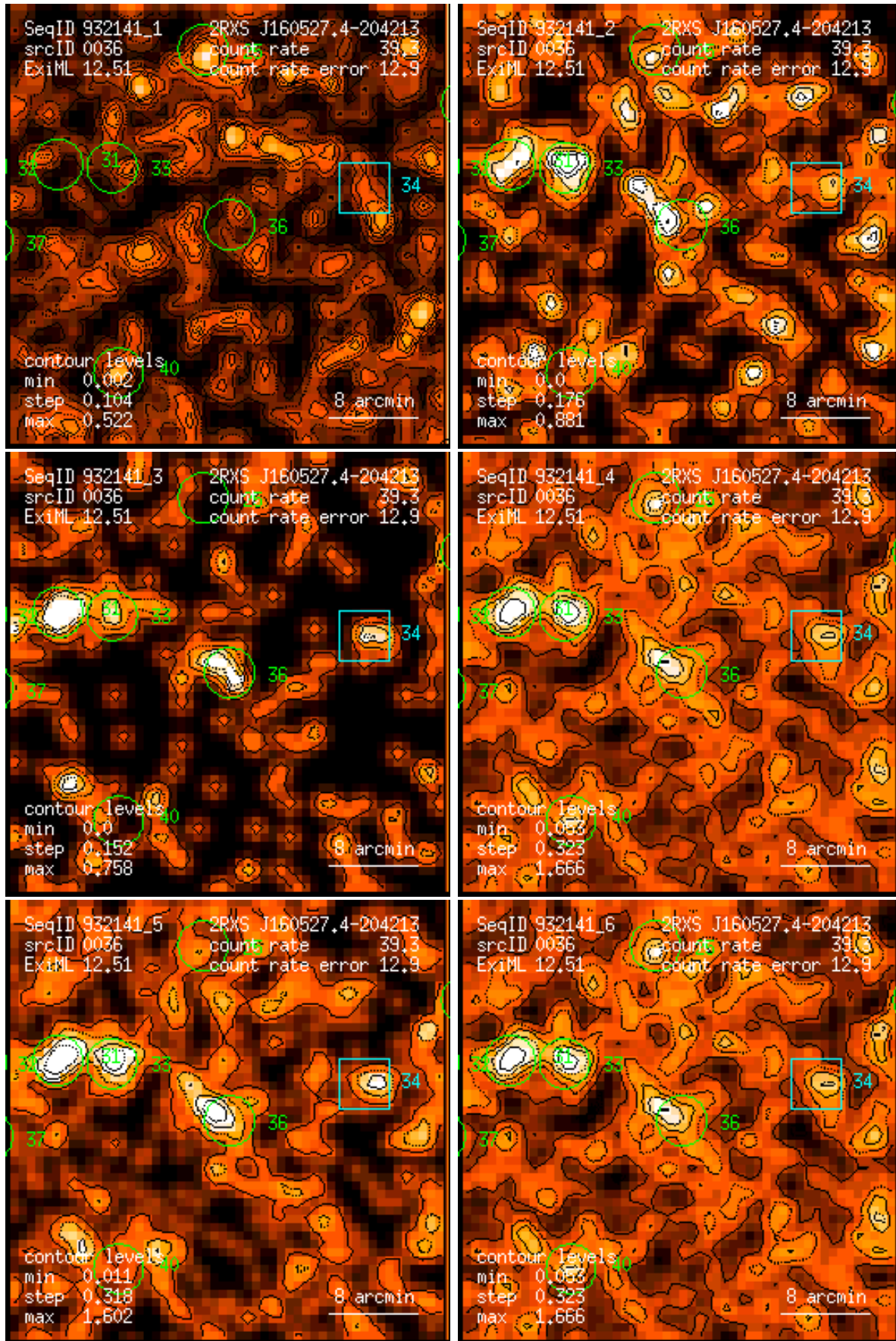
Figure 36: RASS 932141: detection 0036: band rate images, Gaussian filter: (1) PSPC channels 11 – 41, (2) 52 – 90, (3) 91 – 201, (4) 11 – 235, (5) 52 – 201, (6) 11 – 201. Broad band rates in counts/ks. Band rate contour levels in counts/ks/arcmin 2 .
