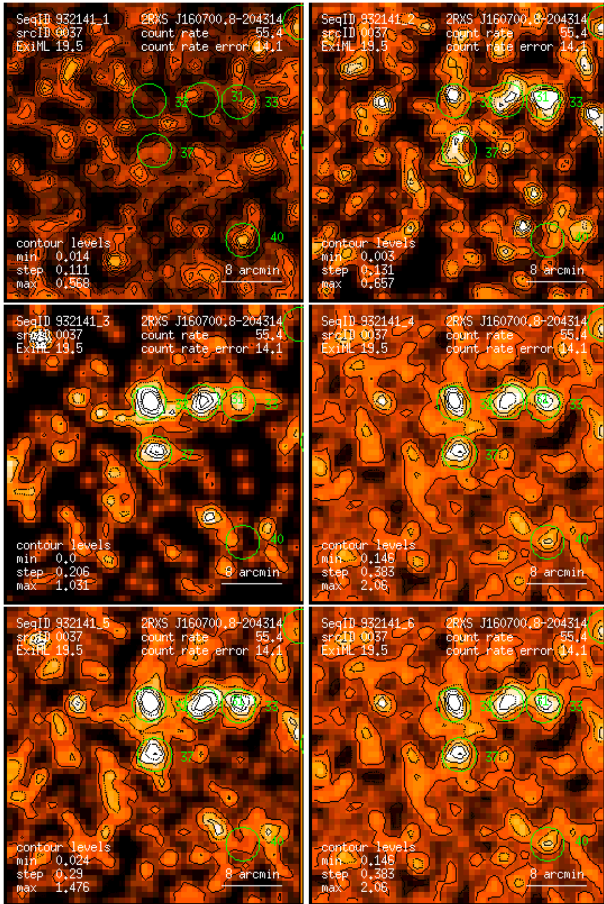
Figure 37: RASS 932141: detection 0037: band rate images, Gaussian filter: (1) PSPC channels 11 – 41, (2) 52 – 90, (3) 91 – 201, (4) 11 – 235, (5) 52 – 201, (6) 11 – 201. Broad band rates in counts/ks. Band rate contour levels in counts/ks/arcmin 2 .
