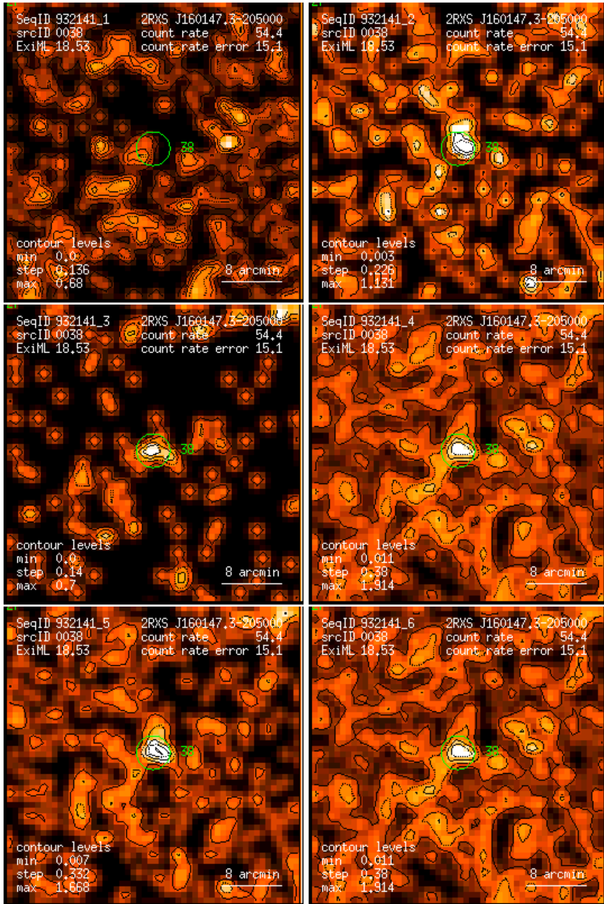
Figure 38: RASS 932141: detection 0038: band rate images, Gaussian filter: (1) PSPC channels 11 – 41, (2) 52 – 90, (3) 91 – 201, (4) 11 – 235, (5) 52 – 201, (6) 11 – 201. Broad band rates in counts/ks. Band rate contour levels in counts/ks/arcmin 2 .
