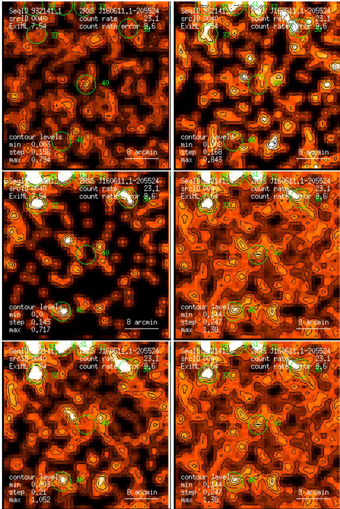
Figure 40: RASS 932141: detection 0040: band rate images, Gaussian filter: (1) PSPC channels 11 – 41, (2) 52 – 90, (3) 91 – 201, (4) 11 – 235, (5) 52 – 201, (6) 11 – 201. Broad band rates in counts/ks. Band rate contour levels in counts/ks/arcmin 2 .
