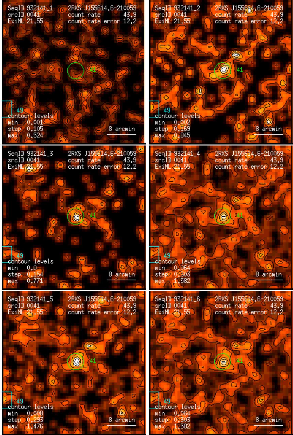
Figure 41: RASS 932141: detection 0041: band rate images, Gaussian filter: (1) PSPC channels 11 – 41, (2) 52 – 90, (3) 91 – 201, (4) 11 – 235, (5) 52 – 201, (6) 11 – 201. Broad band rates in counts/ks. Band rate contour levels in counts/ks/arcmin 2 .
