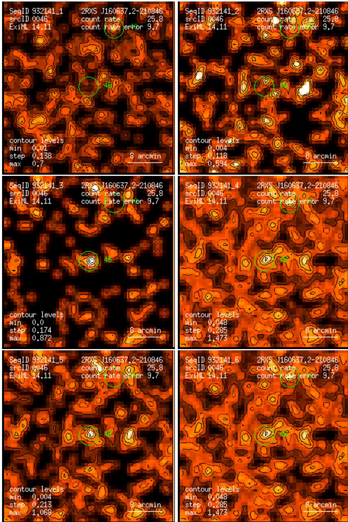
Figure 46: RASS 932141: detection 0046: band rate images, Gaussian filter: (1) PSPC channels 11 – 41, (2) 52 – 90, (3) 91 – 201, (4) 11 – 235, (5) 52 – 201, (6) 11 – 201. Broad band rates in counts/ks. Band rate contour levels in counts/ks/arcmin 2 .
