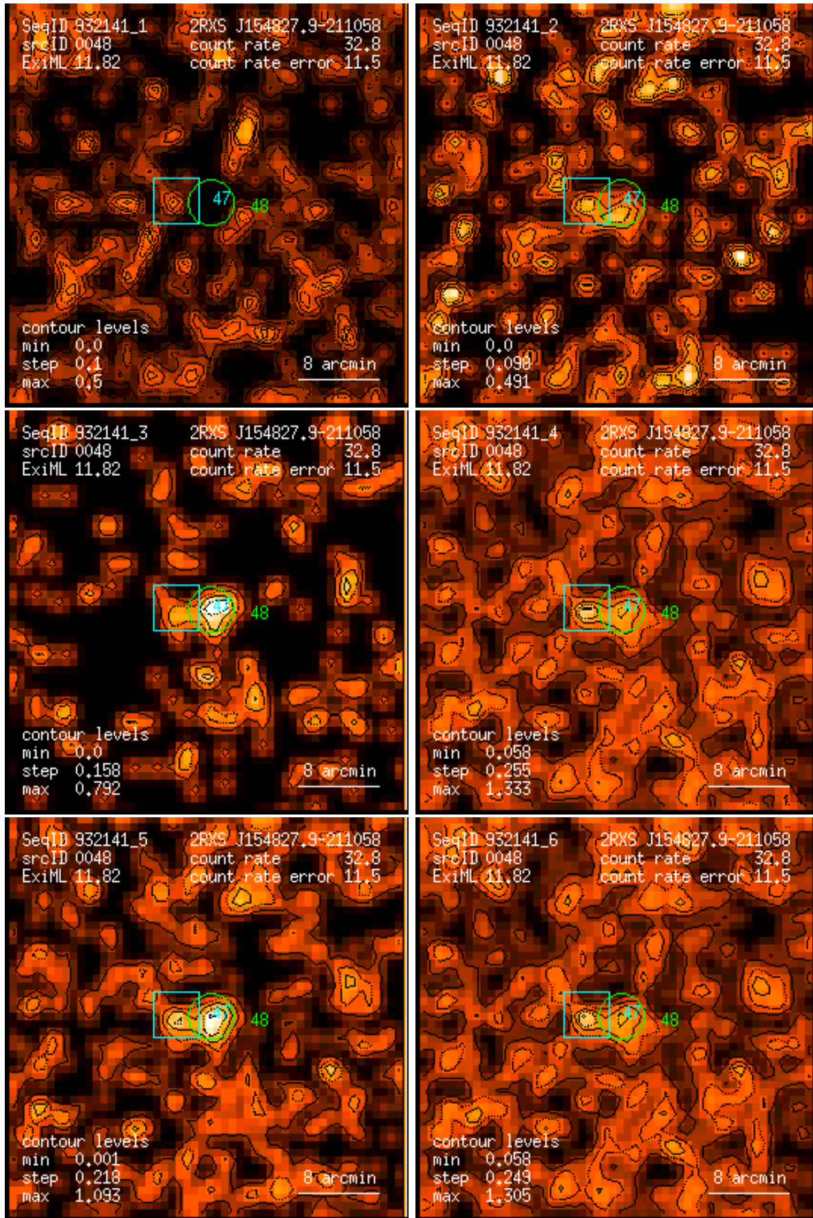
Figure 48: RASS 932141: detection 0048: band rate images, Gaussian filter: (1) PSPC channels 11 – 41, (2) 52 – 90, (3) 91 – 201, (4) 11 – 235, (5) 52 – 201, (6) 11 – 201. Broad band rates in counts/ks. Band rate contour levels in counts/ks/arcmin 2 .
