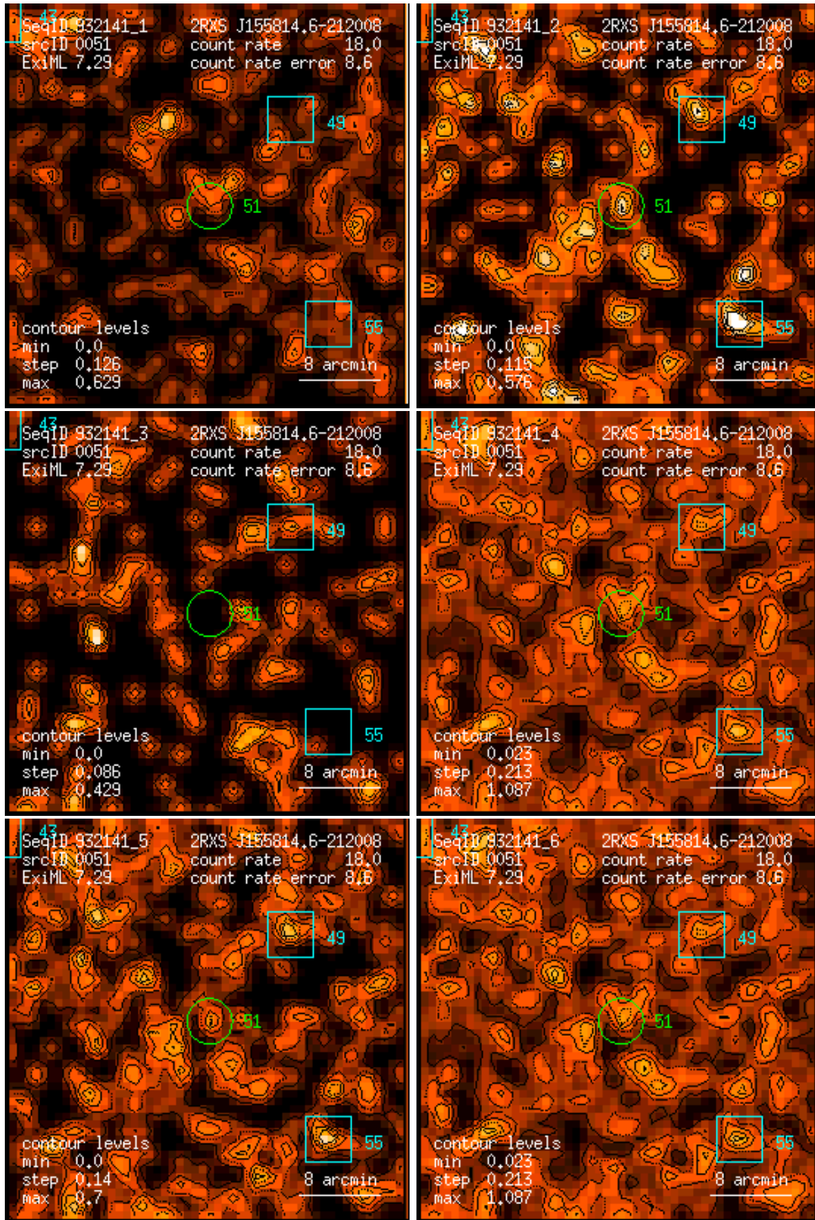
Figure 51: RASS 932141: detection 0051: band rate images, Gaussian filter: (1) PSPC channels 11 – 41, (2) 52 – 90, (3) 91 – 201, (4) 11 – 235, (5) 52 – 201, (6) 11 – 201. Broad band rates in counts/ks. Band rate contour levels in counts/ks/arcmin 2 .
