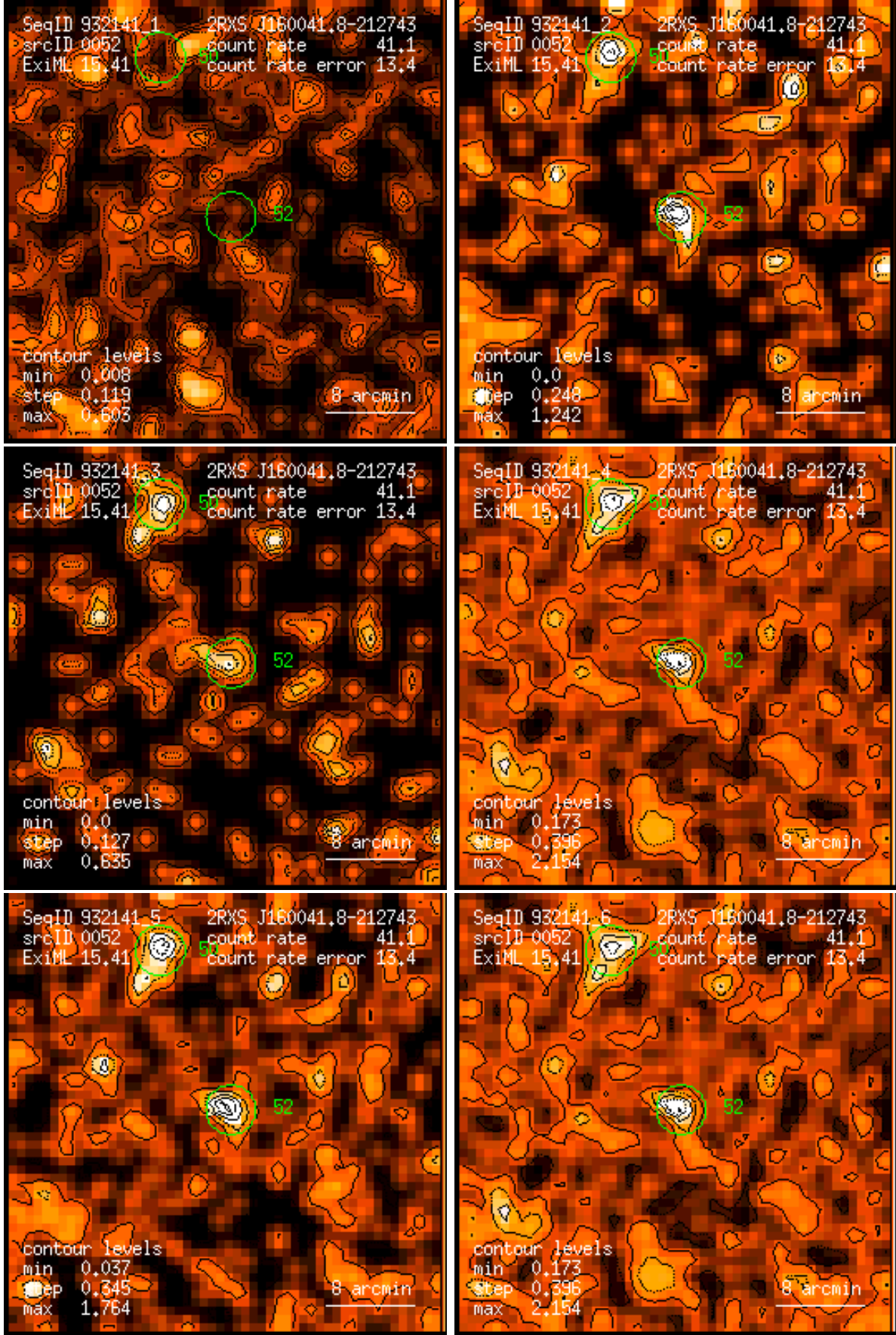
Figure 52: RASS 932141: detection 0052: band rate images, Gaussian filter: (1) PSPC channels 11 – 41, (2) 52 – 90, (3) 91 – 201, (4) 11 – 235, (5) 52 – 201, (6) 11 – 201. Broad band rates in counts/ks. Band rate contour levels in counts/ks/arcmin 2 .
