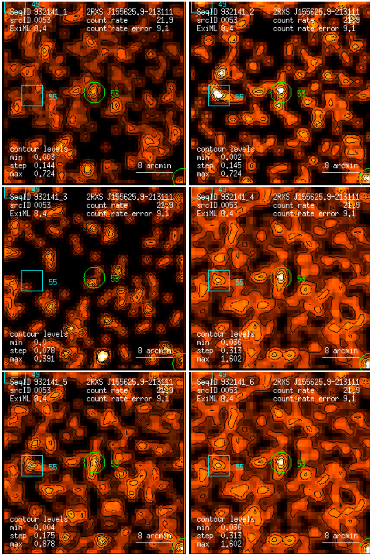
Figure 53: RASS 932141: detection 0053: band rate images, Gaussian filter: (1) PSPC channels 11 – 41, (2) 52 – 90, (3) 91 – 201, (4) 11 – 235, (5) 52 – 201, (6) 11 – 201. Broad band rates in counts/ks. Band rate contour levels in counts/ks/arcmin 2 .
