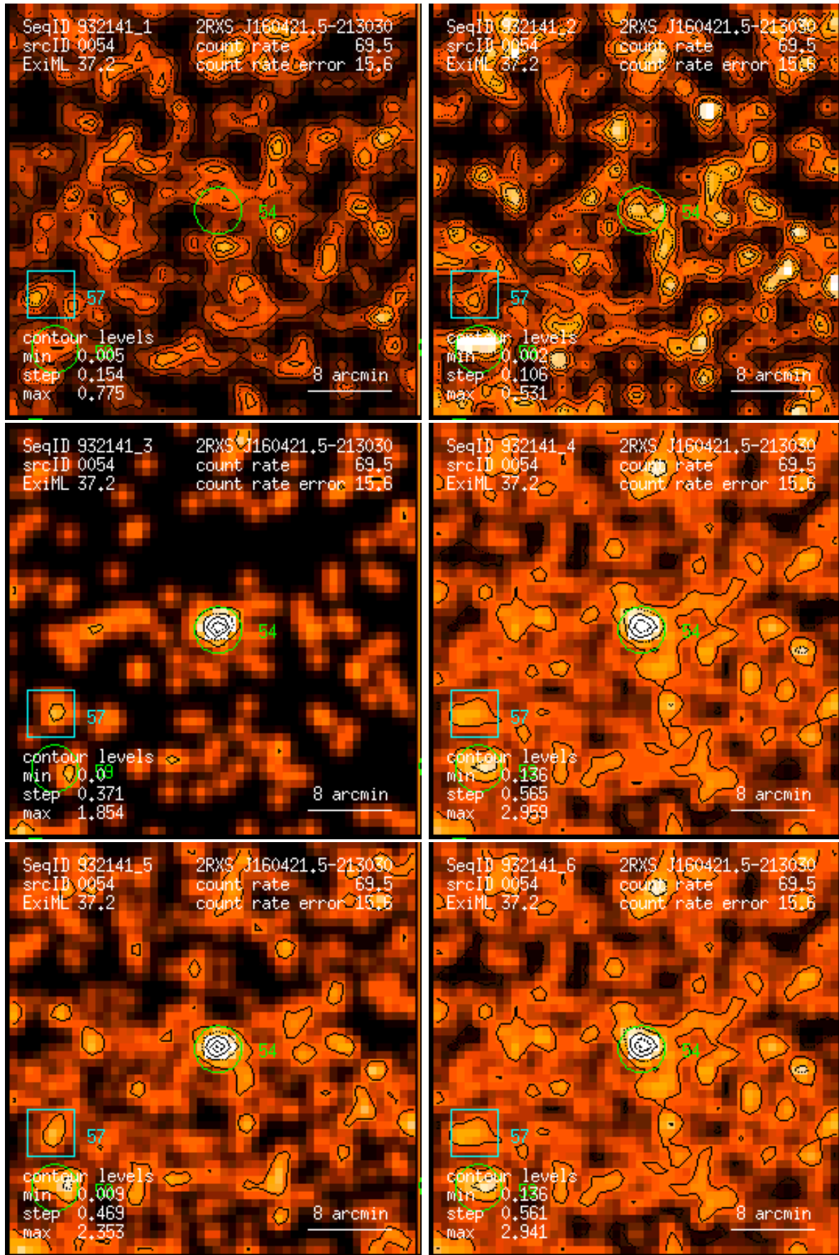
Figure 54: RASS 932141: detection 0054: band rate images, Gaussian filter: (1) PSPC channels 11 – 41, (2) 52 – 90, (3) 91 – 201, (4) 11 – 235, (5) 52 – 201, (6) 11 – 201. Broad band rates in counts/ks. Band rate contour levels in counts/ks/arcmin 2 .
