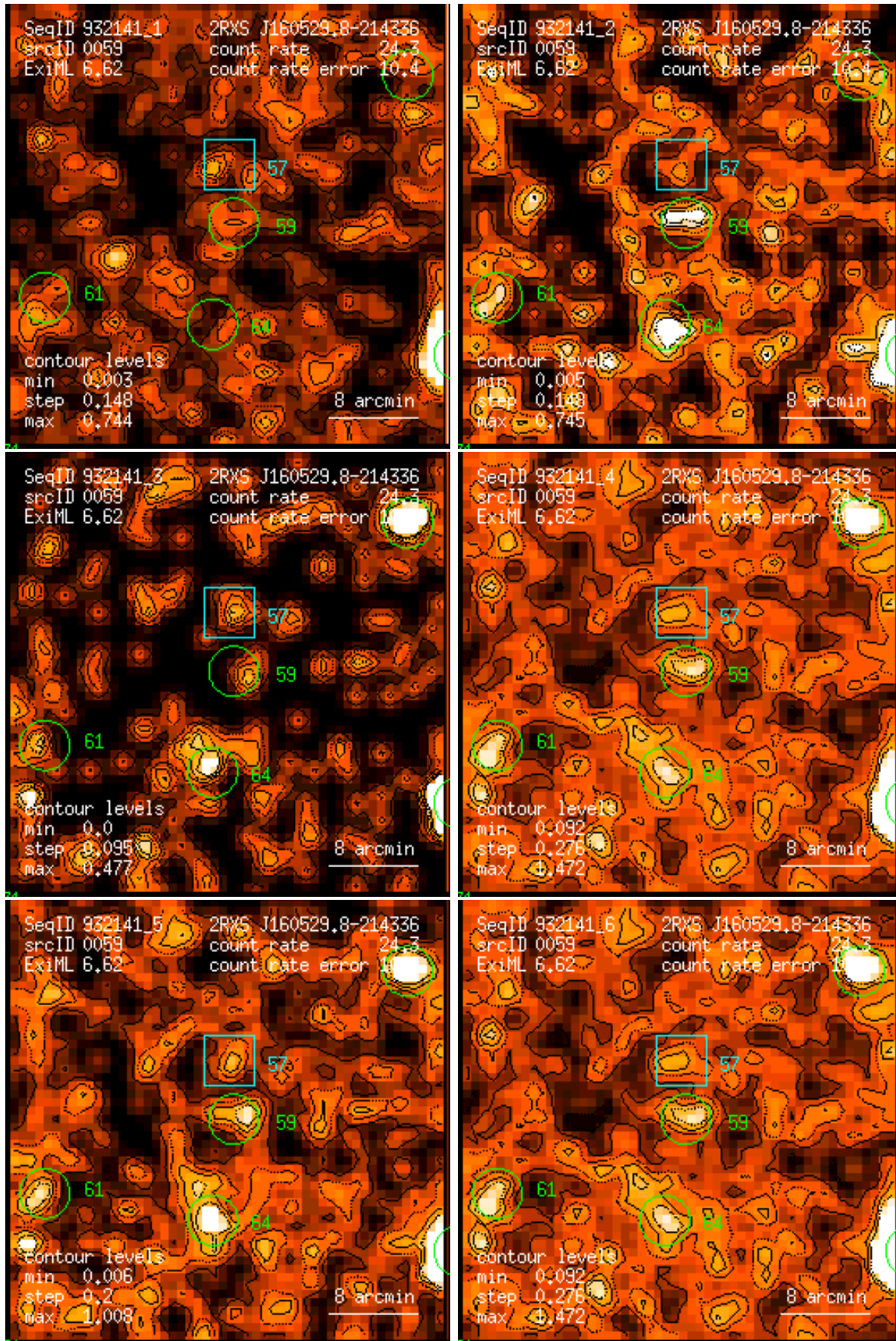
Figure 59: RASS 932141: detection 0059: band rate images, Gaussian filter: (1) PSPC channels 11 – 41, (2) 52 – 90, (3) 91 – 201, (4) 11 – 235, (5) 52 – 201, (6) 11 – 201. Broad band rates in counts/ks. Band rate contour levels in counts/ks/arcmin 2 .
