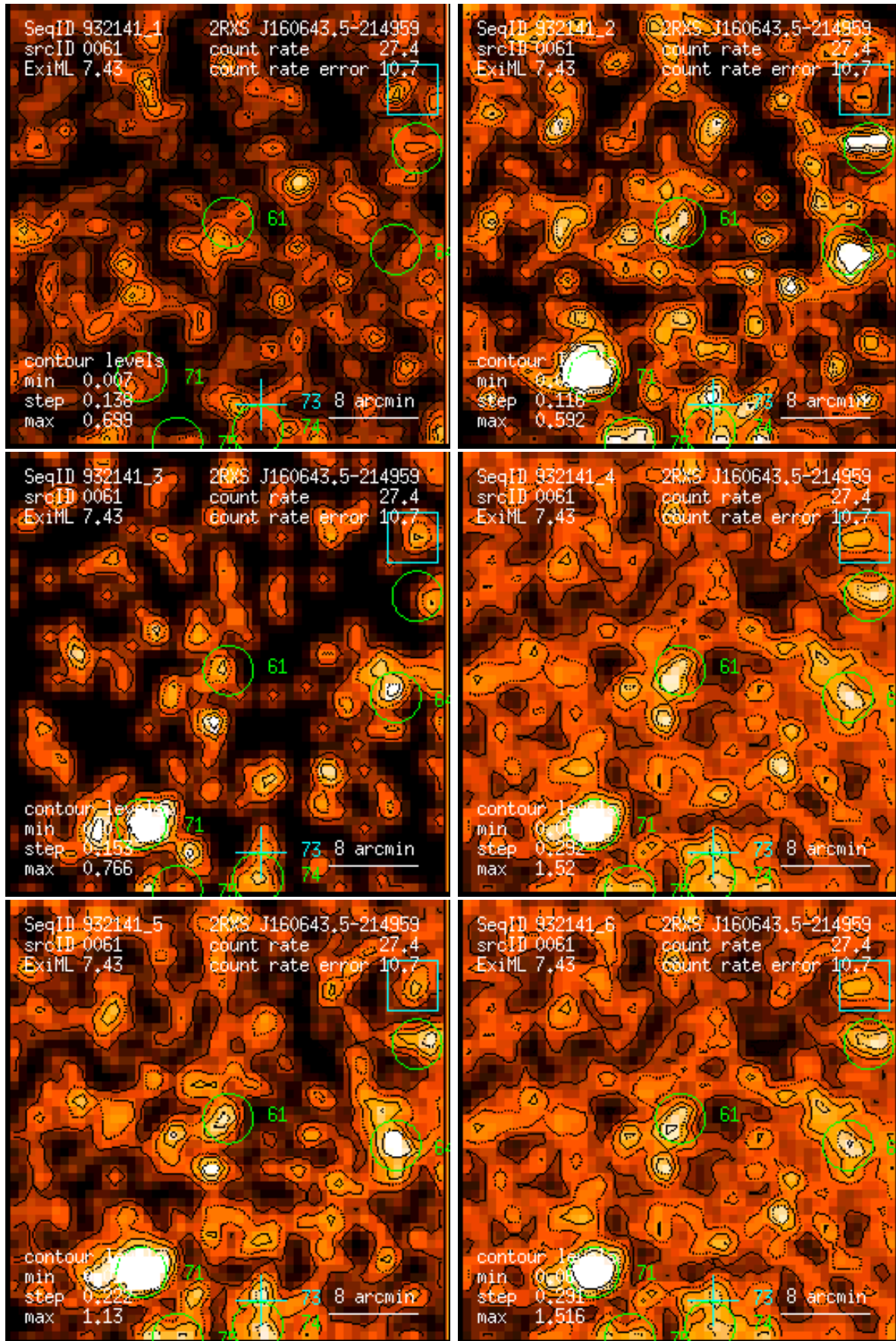
Figure 61: RASS 932141: detection 0061: band rate images, Gaussian filter: (1) PSPC channels 11 – 41, (2) 52 – 90, (3) 91 – 201, (4) 11 – 235, (5) 52 – 201, (6) 11 – 201. Broad band rates in counts/ks. Band rate contour levels in counts/ks/arcmin 2 .
