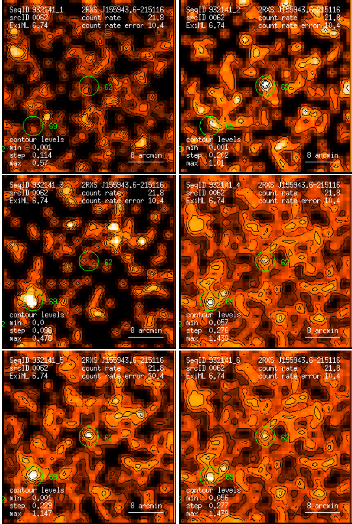
Figure 62: RASS 932141: detection 0062: band rate images, Gaussian filter: (1) PSPC channels 11 – 41, (2) 52 – 90, (3) 91 – 201, (4) 11 – 235, (5) 52 – 201, (6) 11 – 201. Broad band rates in counts/ks. Band rate contour levels in counts/ks/arcmin 2 .
