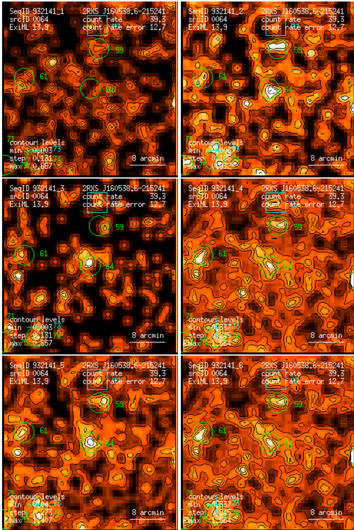
Figure 64: RASS 932141: detection 0064: band rate images, Gaussian filter: (1) PSPC channels 11 – 41, (2) 52 – 90, (3) 91 – 201, (4) 11 – 235, (5) 52 – 201, (6) 11 – 201. Broad band rates in counts/ks. Band rate contour levels in counts/ks/arcmin 2 .
