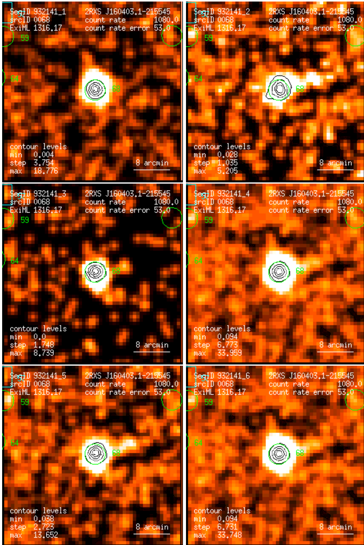
Figure 68: RASS 932141: detection 0068: band rate images, Gaussian filter: (1) PSPC channels 11 – 41, (2) 52 – 90, (3) 91 – 201, (4) 11 – 235, (5) 52 – 201, (6) 11 – 201. Broad band rates in counts/ks. Band rate contour levels in counts/ks/arcmin 2 .
