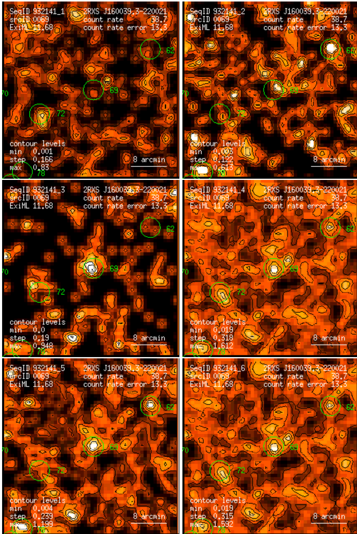
Figure 69: RASS 932141: detection 0069: band rate images, Gaussian filter: (1) PSPC channels 11 – 41, (2) 52 – 90, (3) 91 – 201, (4) 11 – 235, (5) 52 – 201, (6) 11 – 201. Broad band rates in counts/ks. Band rate contour levels in counts/ks/arcmin 2 .
