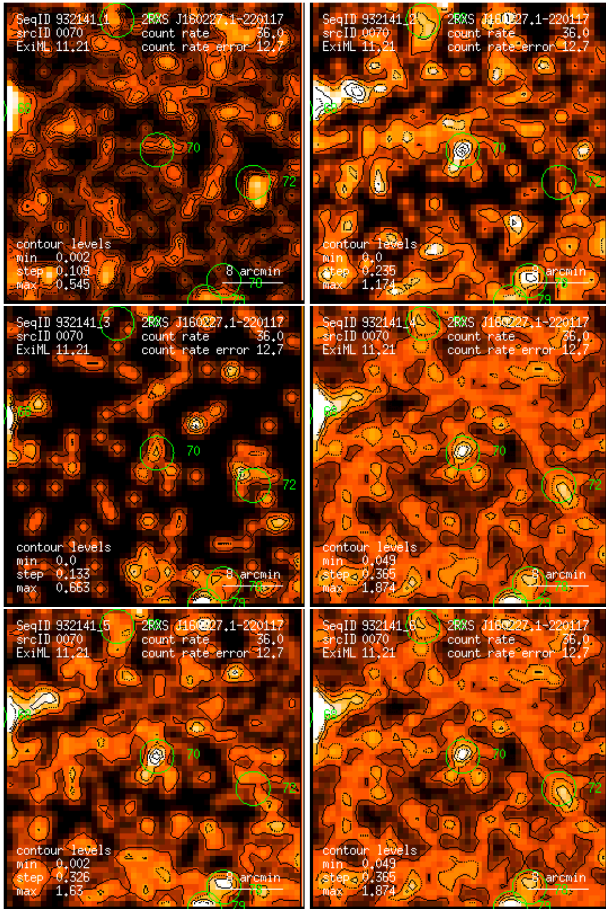
Figure 70: RASS 932141: detection 0070: band rate images, Gaussian filter: (1) PSPC channels 11 – 41, (2) 52 – 90, (3) 91 – 201, (4) 11 – 235, (5) 52 – 201, (6) 11 – 201. Broad band rates in counts/ks. Band rate contour levels in counts/ks/arcmin 2 .
