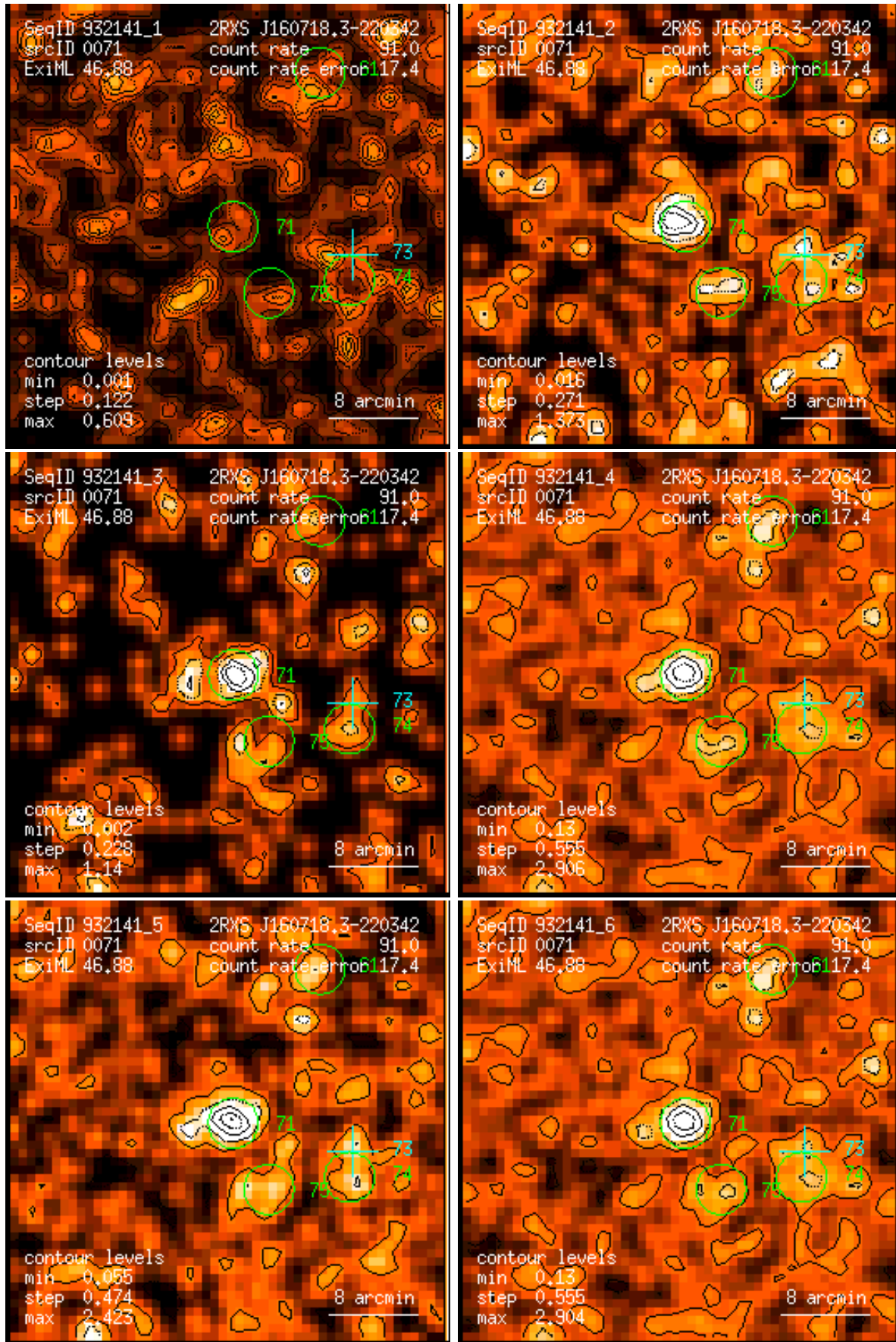
Figure 71: RASS 932141: detection 0071: band rate images, Gaussian filter: (1) PSPC channels 11 – 41, (2) 52 – 90, (3) 91 – 201, (4) 11 – 235, (5) 52 – 201, (6) 11 – 201. Broad band rates in counts/ks. Band rate contour levels in counts/ks/arcmin 2 .
