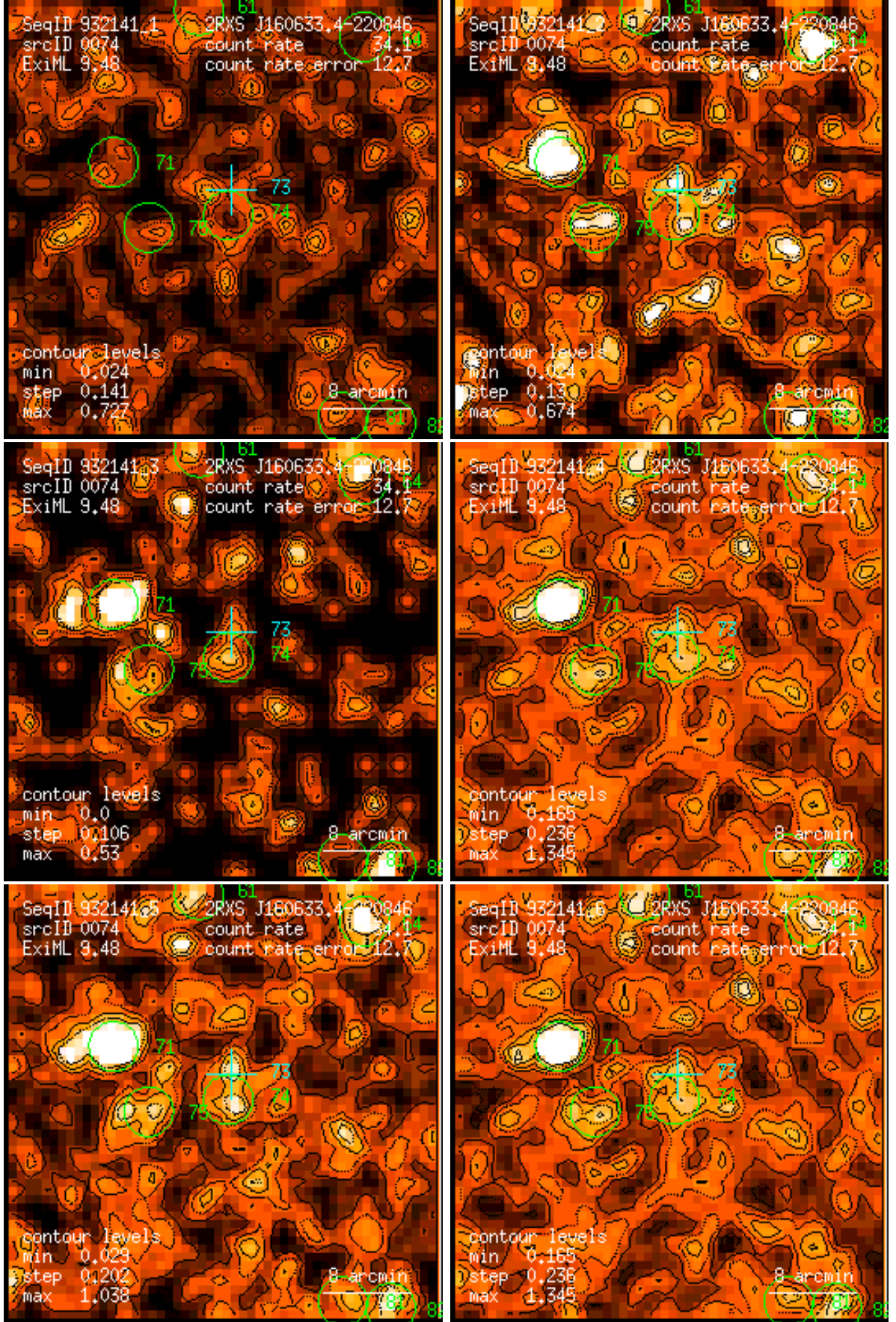
Figure 74: RASS 932141: detection 0074: band rate images, Gaussian filter: (1) PSPC channels 11 – 41, (2) 52 – 90, (3) 91 – 201, (4) 11 – 235, (5) 52 – 201, (6) 11 – 201. Broad band rates in counts/ks. Band rate contour levels in counts/ks/arcmin 2 .
