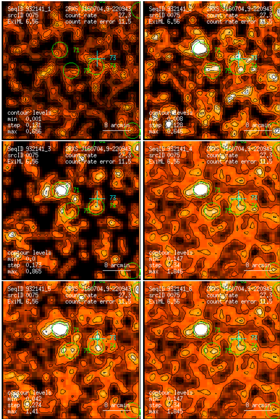
Figure 75: RASS 932141: detection 0075: band rate images, Gaussian filter: (1) PSPC channels 11 – 41, (2) 52 – 90, (3) 91 – 201, (4) 11 – 235, (5) 52 – 201, (6) 11 – 201. Broad band rates in counts/ks. Band rate contour levels in counts/ks/arcmin 2 .
