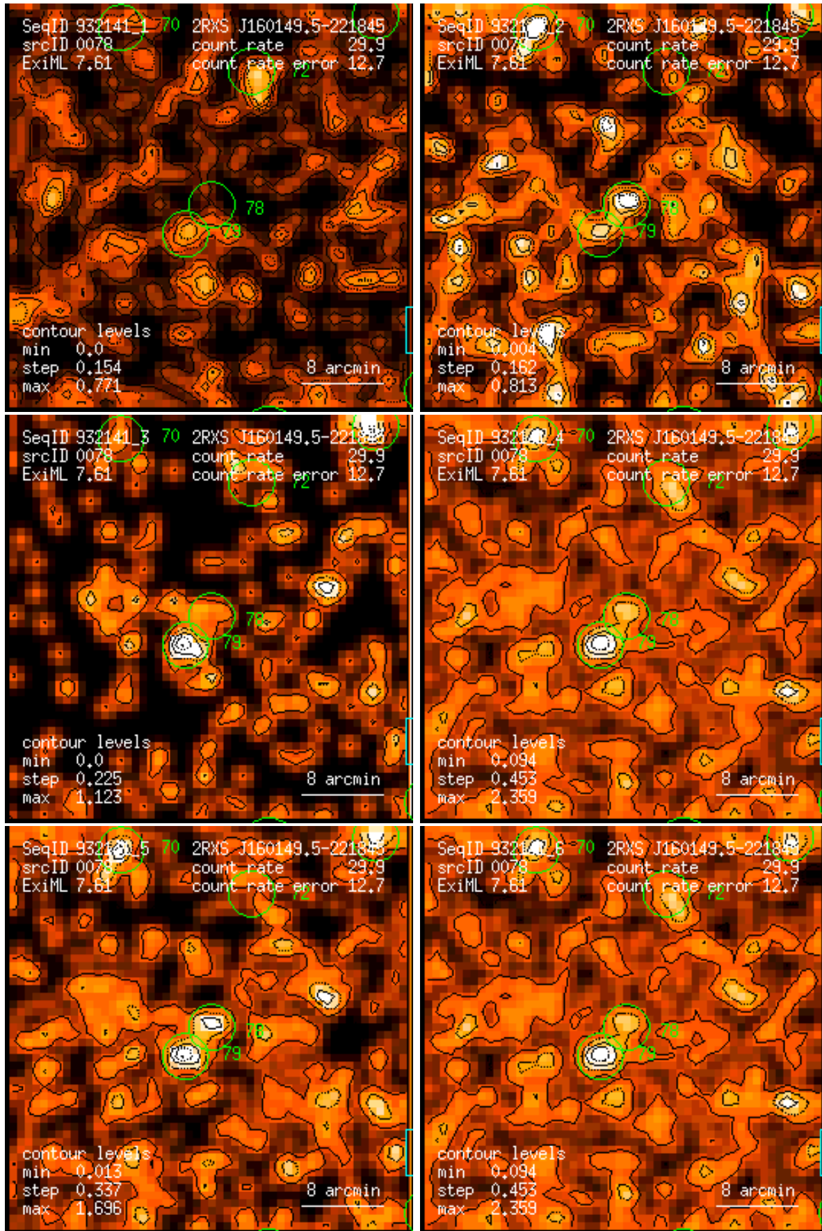
Figure 78: RASS 932141: detection 0078: band rate images, Gaussian filter: (1) PSPC channels 11 – 41, (2) 52 – 90, (3) 91 – 201, (4) 11 – 235, (5) 52 – 201, (6) 11 – 201. Broad band rates in counts/ks. Band rate contour levels in counts/ks/arcmin 2 .
