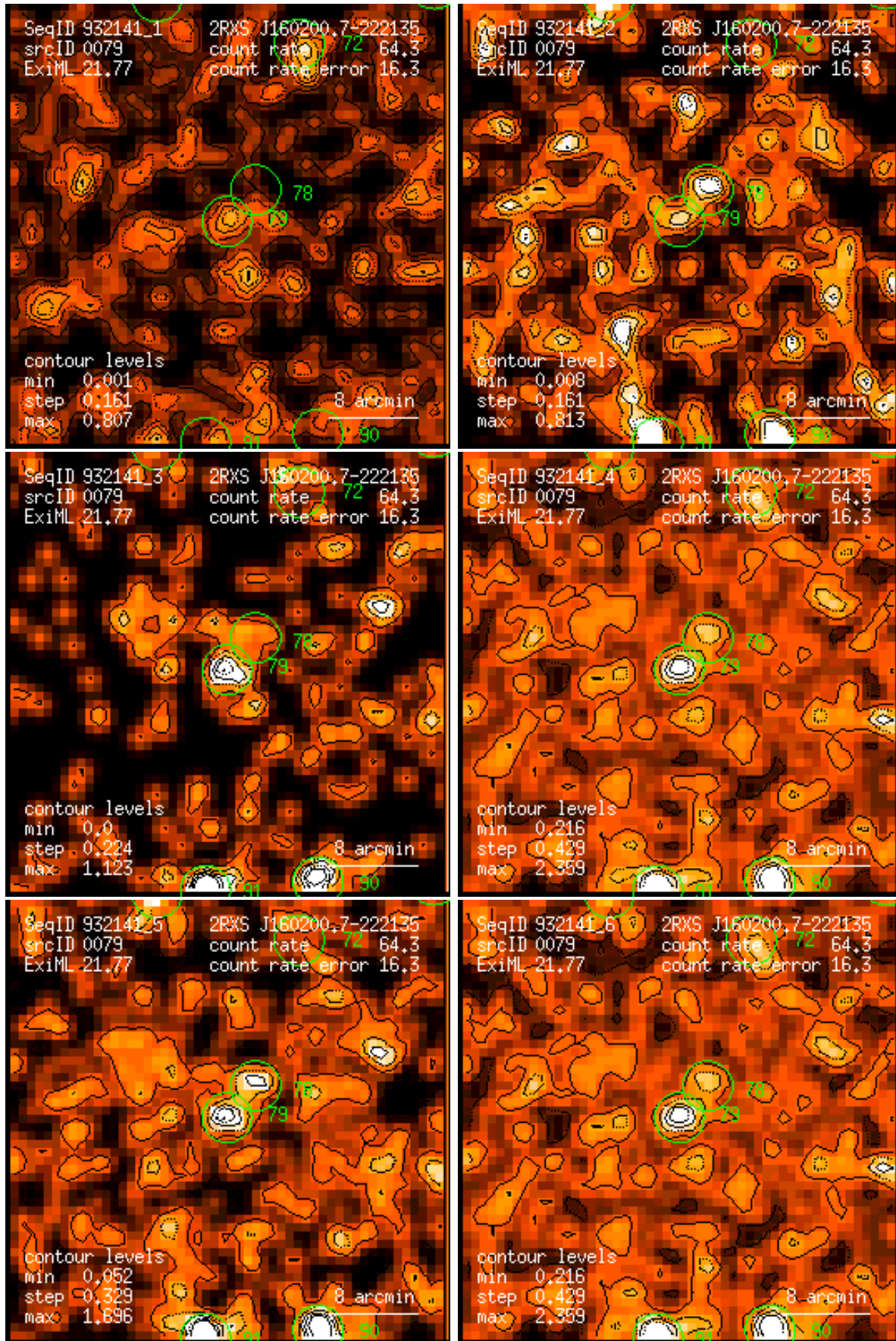
Figure 79: RASS 932141: detection 0079: band rate images, Gaussian filter: (1) PSPC channels 11 – 41, (2) 52 – 90, (3) 91 – 201, (4) 11 – 235, (5) 52 – 201, (6) 11 – 201. Broad band rates in counts/ks. Band rate contour levels in counts/ks/arcmin 2 .
