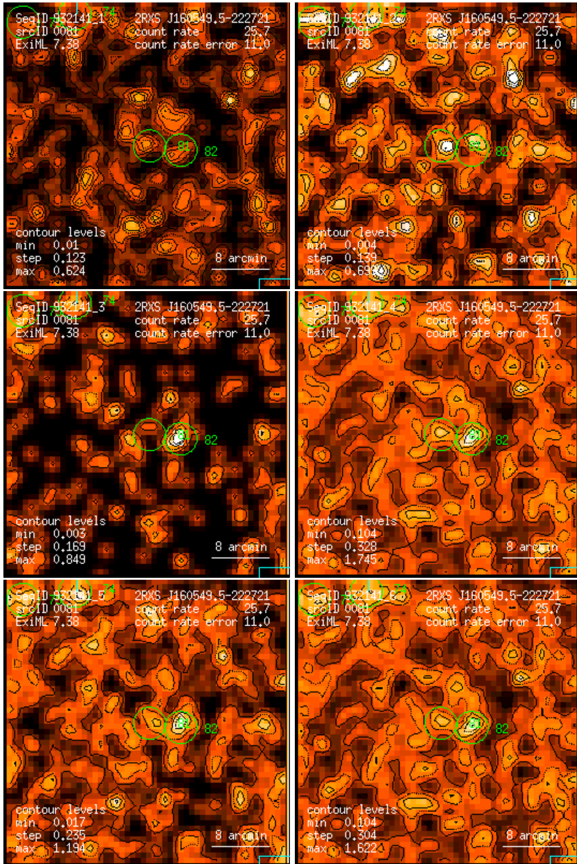
Figure 81: RASS 932141: detection 0081: band rate images, Gaussian filter: (1) PSPC channels 11 – 41, (2) 52 – 90, (3) 91 – 201, (4) 11 – 235, (5) 52 – 201, (6) 11 – 201. Broad band rates in counts/ks. Band rate contour levels in counts/ks/arcmin 2 .
