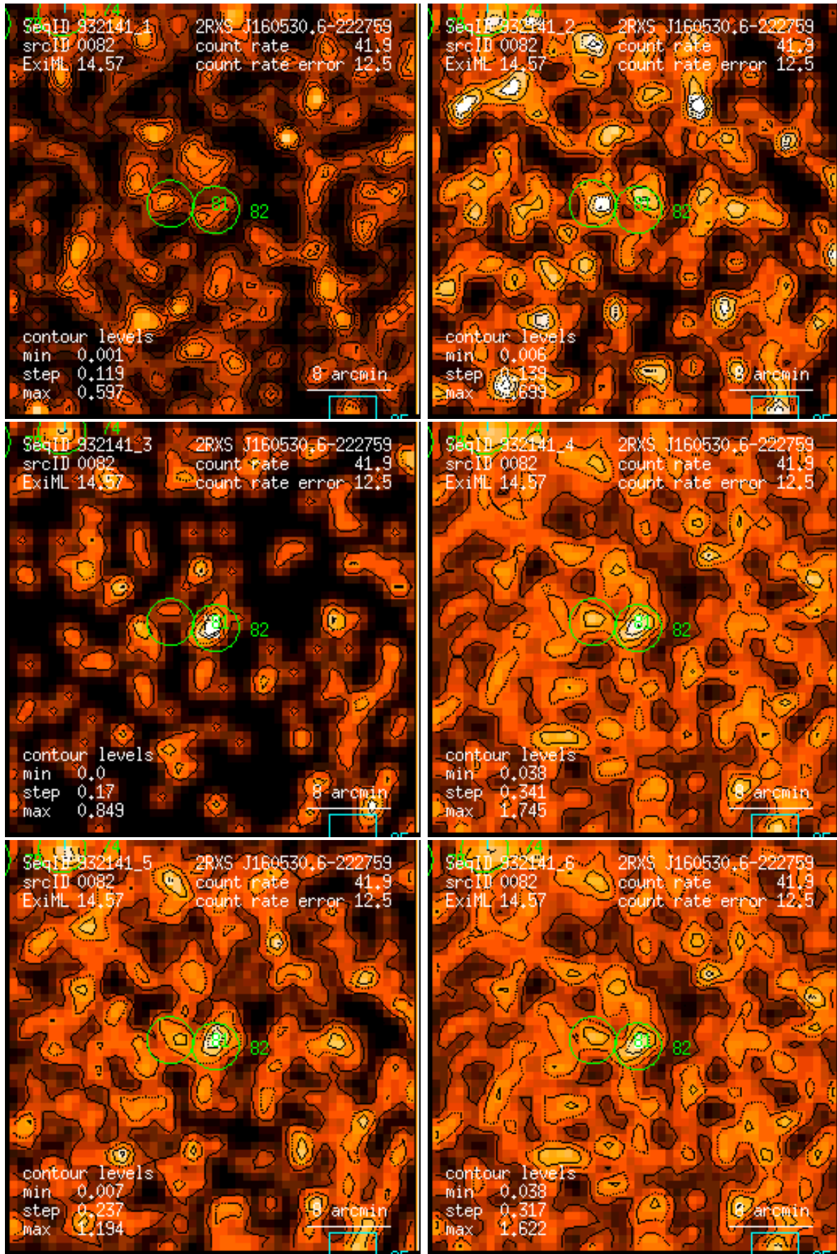
Figure 82: RASS 932141: detection 0082: band rate images, Gaussian filter: (1) PSPC channels 11 – 41, (2) 52 – 90, (3) 91 – 201, (4) 11 – 235, (5) 52 – 201, (6) 11 – 201. Broad band rates in counts/ks. Band rate contour levels in counts/ks/arcmin 2 .
