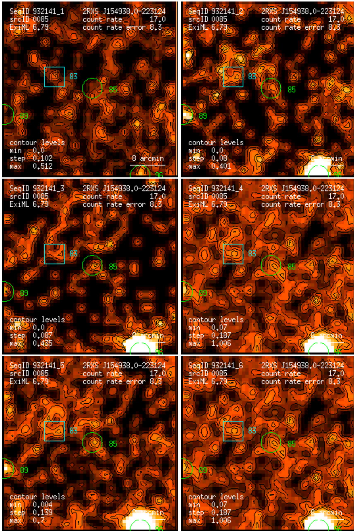
Figure 85: RASS 932141: detection 0085: band rate images, Gaussian filter: (1) PSPC channels 11 – 41, (2) 52 – 90, (3) 91 – 201, (4) 11 – 235, (5) 52 – 201, (6) 11 – 201. Broad band rates in counts/ks. Band rate contour levels in counts/ks/arcmin 2 .
