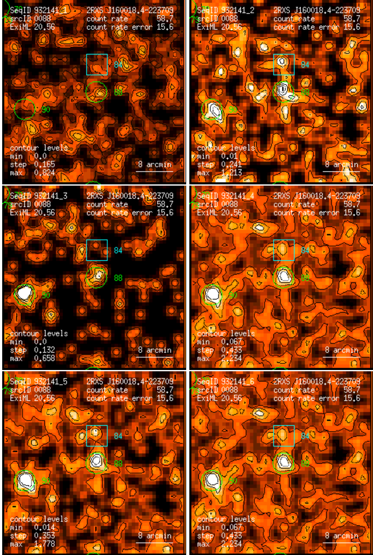
Figure 88: RASS 932141: detection 0088: band rate images, Gaussian filter: (1) PSPC channels 11 – 41, (2) 52 – 90, (3) 91 – 201, (4) 11 – 235, (5) 52 – 201, (6) 11 – 201. Broad band rates in counts/ks. Band rate contour levels in counts/ks/arcmin 2 .
