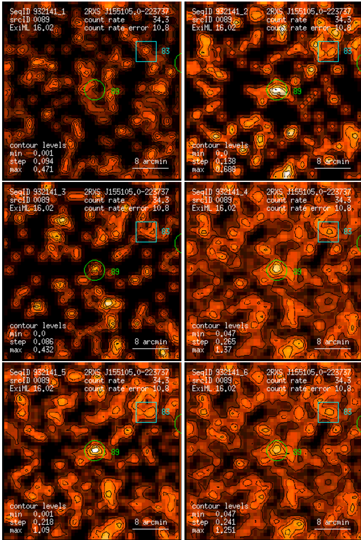
Figure 89: RASS 932141: detection 0089: band rate images, Gaussian filter: (1) PSPC channels 11 – 41, (2) 52 – 90, (3) 91 – 201, (4) 11 – 235, (5) 52 – 201, (6) 11 – 201. Broad band rates in counts/ks. Band rate contour levels in counts/ks/arcmin 2 .
