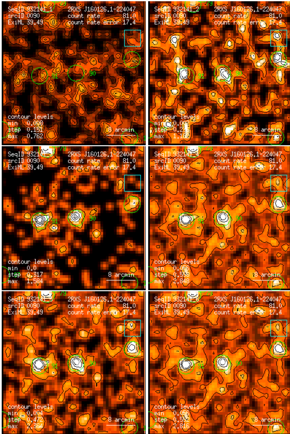
Figure 90: RASS 932141: detection 0090: band rate images, Gaussian filter: (1) PSPC channels 11 – 41, (2) 52 – 90, (3) 91 – 201, (4) 11 – 235, (5) 52 – 201, (6) 11 – 201. Broad band rates in counts/ks. Band rate contour levels in counts/ks/arcmin 2 .
