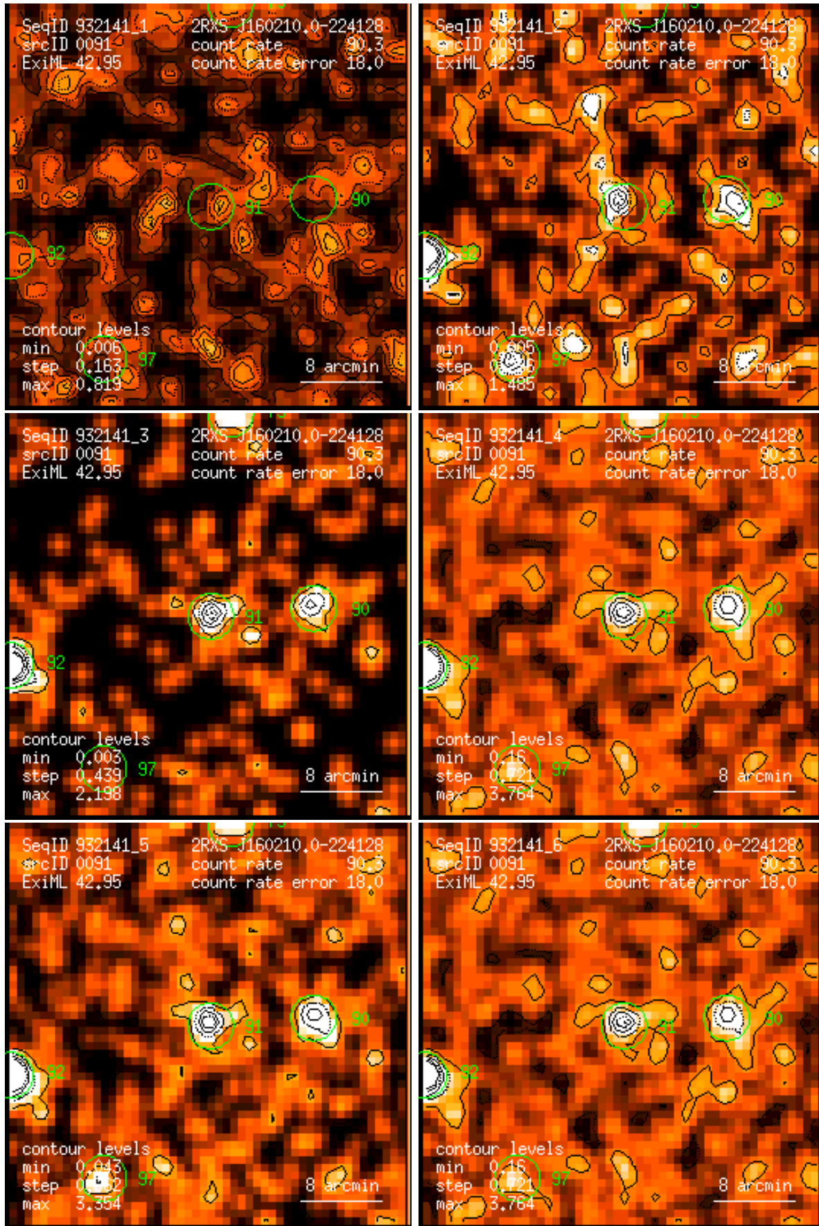
Figure 91: RASS 932141: detection 0091: band rate images, Gaussian filter: (1) PSPC channels 11 – 41, (2) 52 – 90, (3) 91 – 201, (4) 11 – 235, (5) 52 – 201, (6) 11 – 201. Broad band rates in counts/ks. Band rate contour levels in counts/ks/arcmin 2 .
