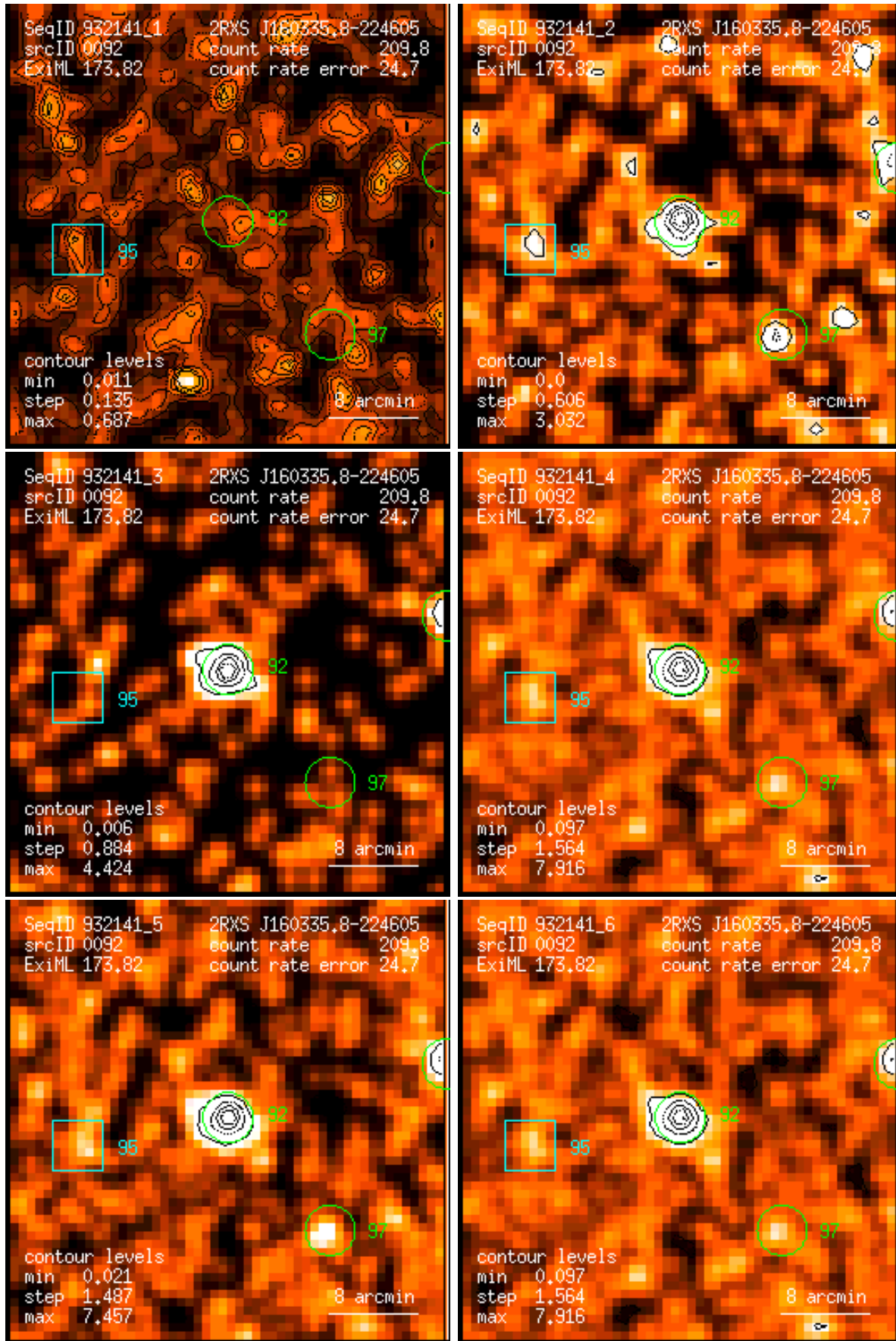
Figure 92: RASS 932141: detection 0092: band rate images, Gaussian filter: (1) PSPC channels 11 – 41, (2) 52 – 90, (3) 91 – 201, (4) 11 – 235, (5) 52 – 201, (6) 11 – 201. Broad band rates in counts/ks. Band rate contour levels in counts/ks/arcmin 2 .
