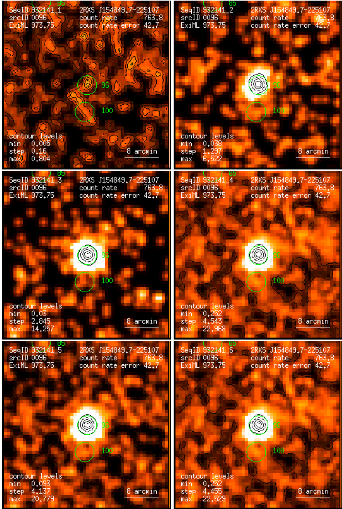
Figure 96: RASS 932141: detection 0096: band rate images, Gaussian filter: (1) PSPC channels 11 – 41, (2) 52 – 90, (3) 91 – 201, (4) 11 – 235, (5) 52 – 201, (6) 11 – 201. Broad band rates in counts/ks. Band rate contour levels in counts/ks/arcmin 2 .
