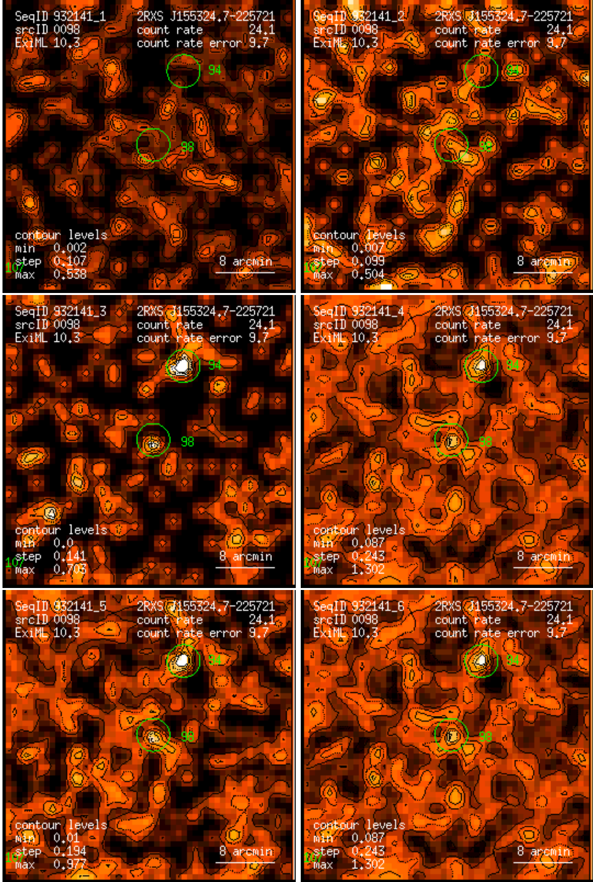
Figure 98: RASS 932141: detection 0098: band rate images, Gaussian filter: (1) PSPC channels 11 – 41, (2) 52 – 90, (3) 91 – 201, (4) 11 – 235, (5) 52 – 201, (6) 11 – 201. Broad band rates in counts/ks. Band rate contour levels in counts/ks/arcmin 2 .
