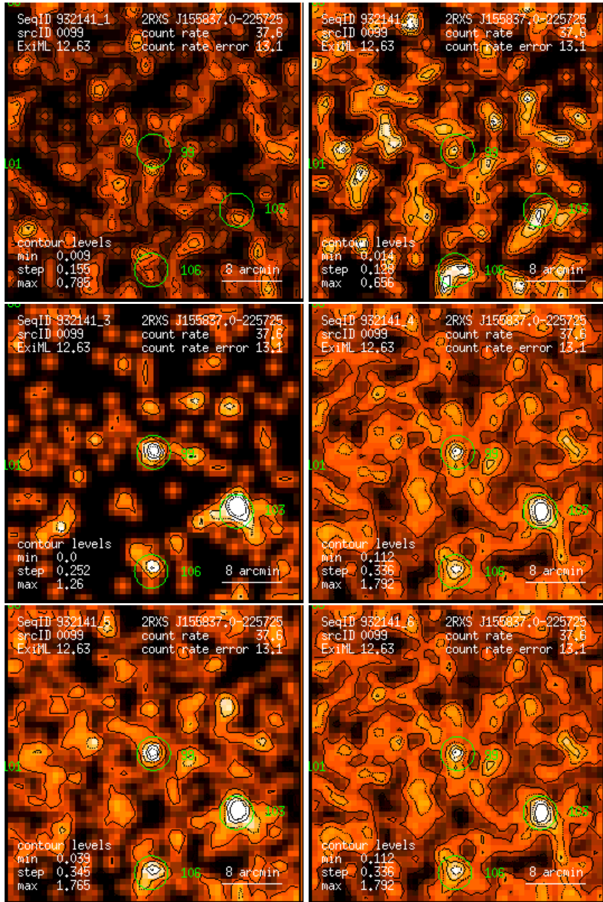
Figure 99: RASS 932141: detection 0099: band rate images, Gaussian filter: (1) PSPC channels 11 – 41, (2) 52 – 90, (3) 91 – 201, (4) 11 – 235, (5) 52 – 201, (6) 11 – 201. Broad band rates in counts/ks. Band rate contour levels in counts/ks/arcmin 2 .
