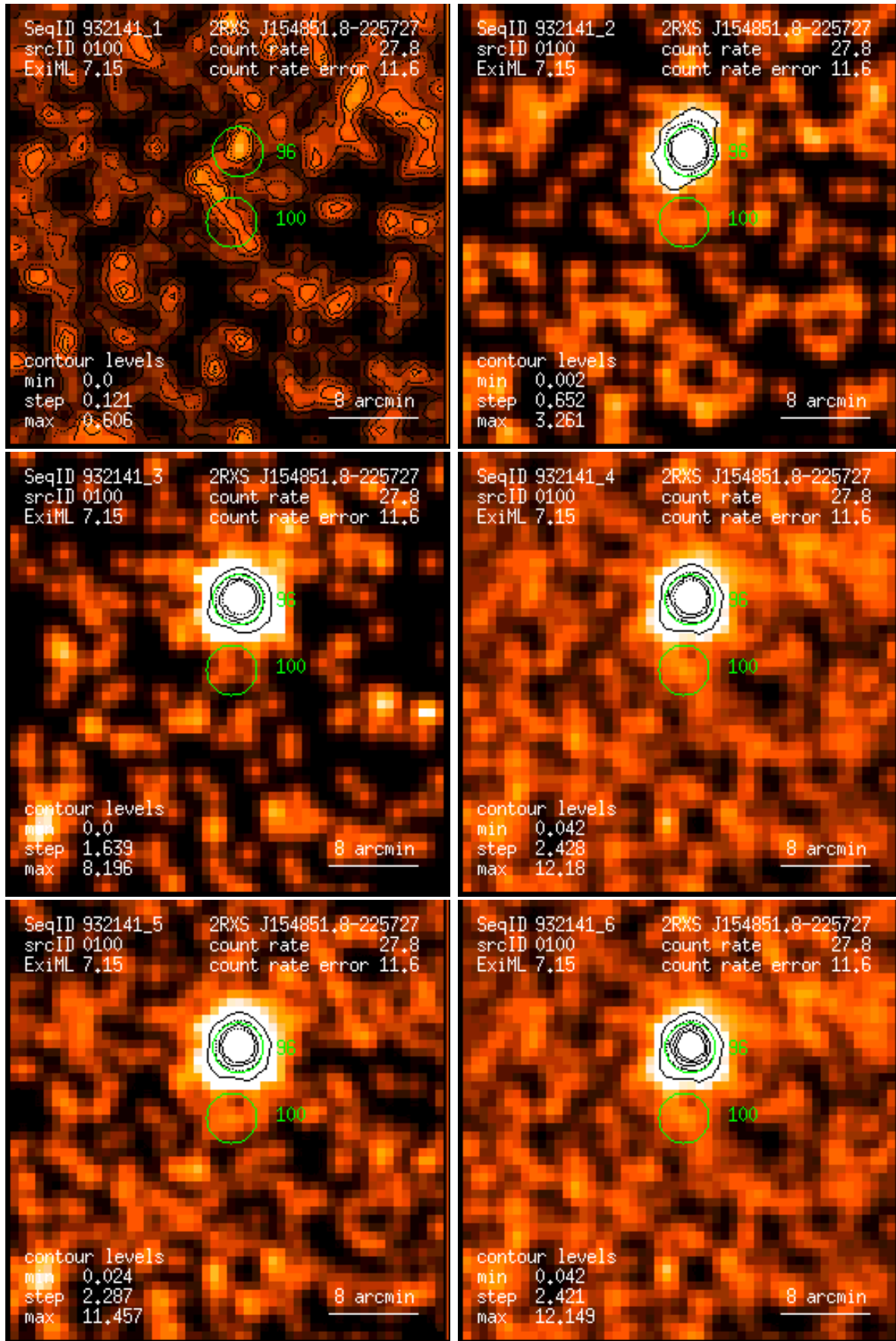
Figure 100: RASS 932141: detection 0100: band rate images, Gaussian filter: (1) PSPC channels 11 – 41, (2) 52 – 90, (3) 91 – 201, (4) 11 – 235, (5) 52 – 201, (6) 11 – 201. Broad band rates in counts/ks. Band rate contour levels in counts/ks/arcmin 2 .
