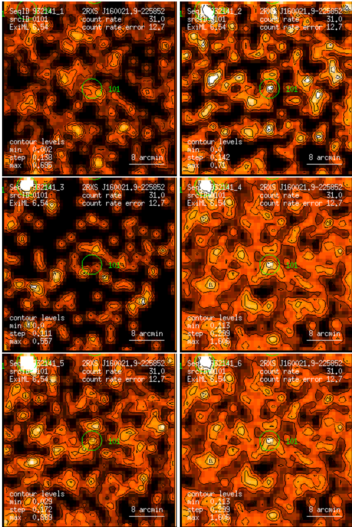
Figure 101: RASS 932141: detection 0101: band rate images, Gaussian filter: (1) PSPC channels 11 – 41, (2) 52 – 90, (3) 91 – 201, (4) 11 – 235, (5) 52 – 201, (6) 11 – 201. Broad band rates in counts/ks. Band rate contour levels in counts/ks/arcmin 2 .
