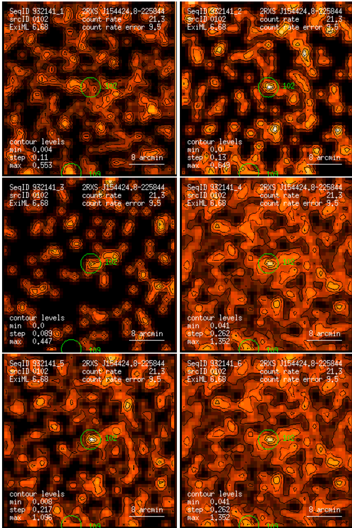
Figure 102: RASS 932141: detection 0102: band rate images, Gaussian filter: (1) PSPC channels 11 – 41, (2) 52 – 90, (3) 91 – 201, (4) 11 – 235, (5) 52 – 201, (6) 11 – 201. Broad band rates in counts/ks. Band rate contour levels in counts/ks/arcmin 2 .
