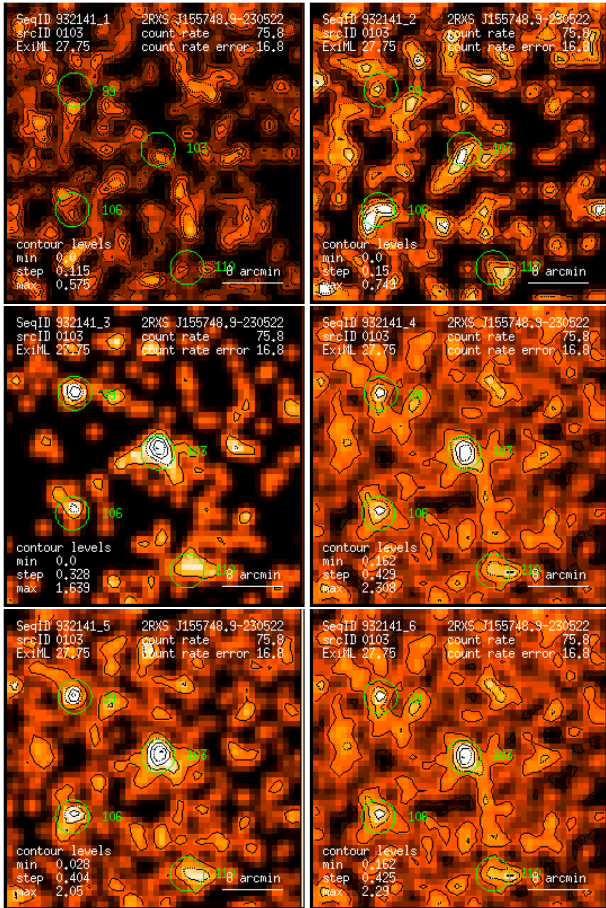
Figure 103: RASS 932141: detection 0103: band rate images, Gaussian filter: (1) PSPC channels 11 – 41, (2) 52 – 90, (3) 91 – 201, (4) 11 – 235, (5) 52 – 201, (6) 11 – 201. Broad band rates in counts/ks. Band rate contour levels in counts/ks/arcmin 2 .
