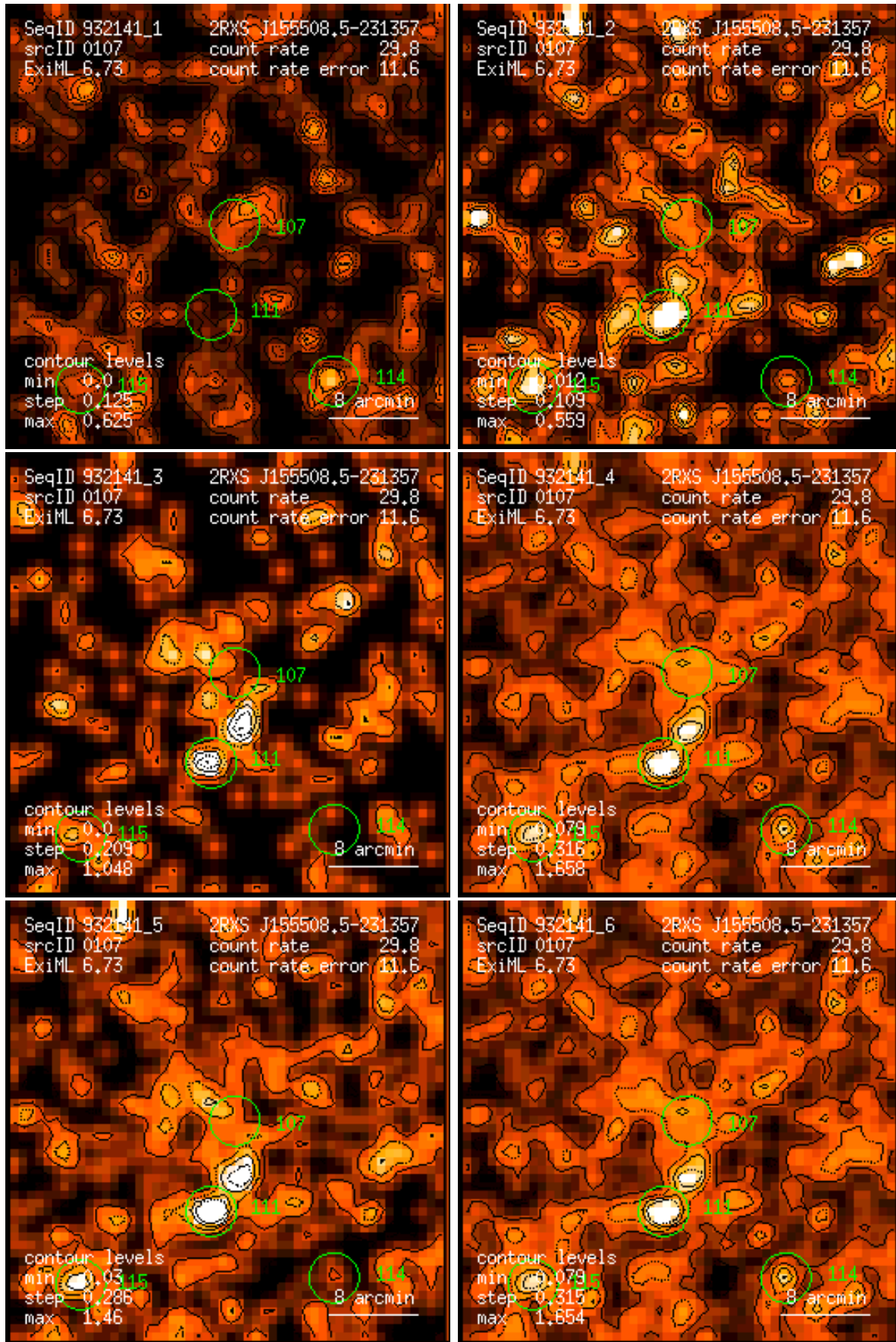
Figure 107: RASS 932141: detection 0107: band rate images, Gaussian filter: (1) PSPC channels 11 – 41, (2) 52 – 90, (3) 91 – 201, (4) 11 – 235, (5) 52 – 201, (6) 11 – 201. Broad band rates in counts/ks. Band rate contour levels in counts/ks/arcmin 2 .
