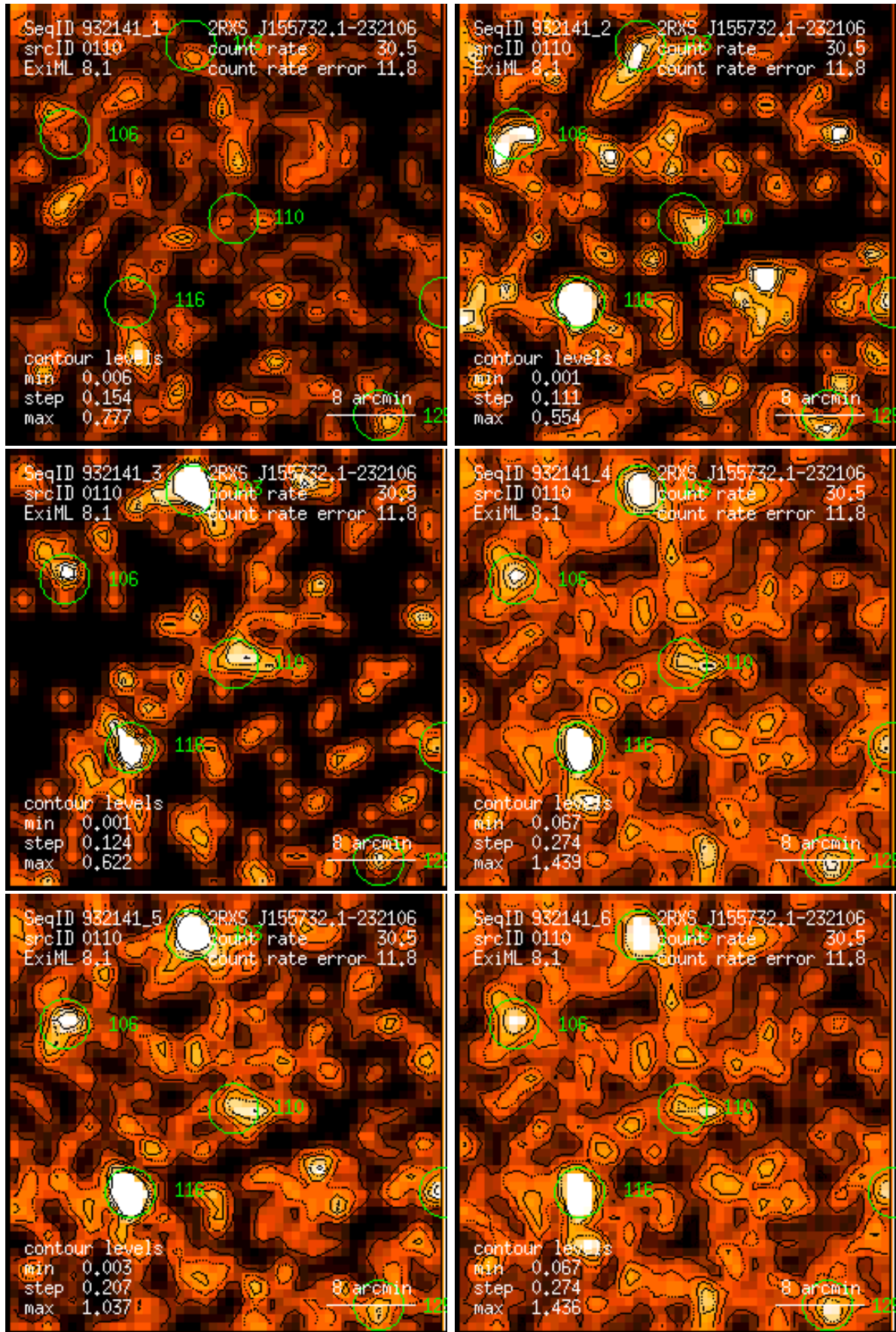
Figure 110: RASS 932141: detection 0110: band rate images, Gaussian filter: (1) PSPC channels 11 – 41, (2) 52 – 90, (3) 91 – 201, (4) 11 – 235, (5) 52 – 201, (6) 11 – 201. Broad band rates in counts/ks. Band rate contour levels in counts/ks/arcmin 2 .
